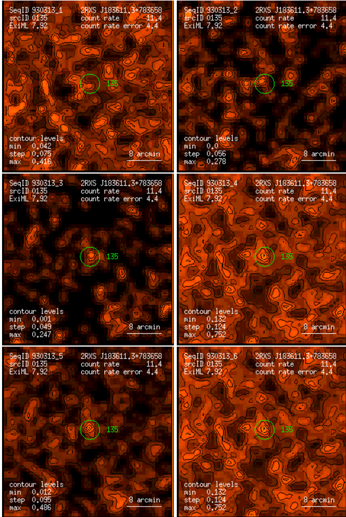
Figure 135: RASS 930313: detection 0135: band rate images, Gaussian filter: (1) PSPC channels 11 – 41, (2) 52 – 90, (3) 91 – 201, (4) 11 – 235, (5) 52 – 201, (6) 11 – 201. Broad band rates in counts/ks. Band rate contour levels in counts/ks/arcmin 2 .
