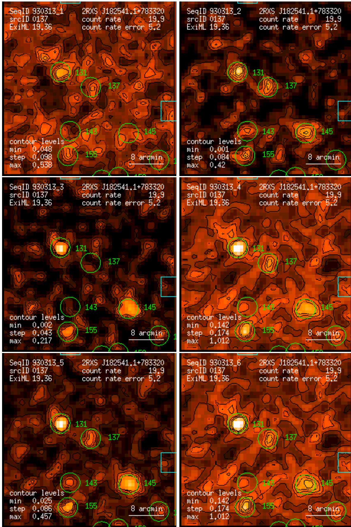
Figure 137: RASS 930313: detection 0137: band rate images, Gaussian filter: (1) PSPC channels 11 – 41, (2) 52 – 90, (3) 91 – 201, (4) 11 – 235, (5) 52 – 201, (6) 11 – 201. Broad band rates in counts/ks. Band rate contour levels in counts/ks/arcmin 2 .
