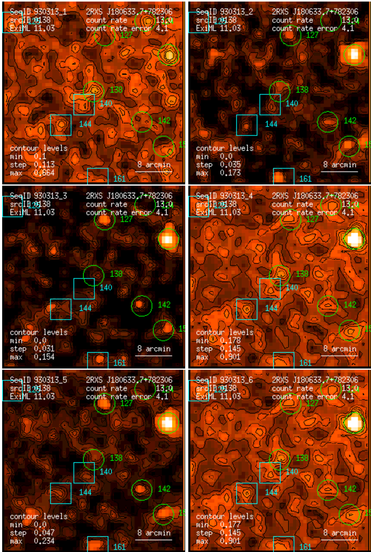
Figure 138: RASS 930313: detection 0138: band rate images, Gaussian filter: (1) PSPC channels 11 – 41, (2) 52 – 90, (3) 91 – 201, (4) 11 – 235, (5) 52 – 201, (6) 11 – 201. Broad band rates in counts/ks. Band rate contour levels in counts/ks/arcmin 2 .
