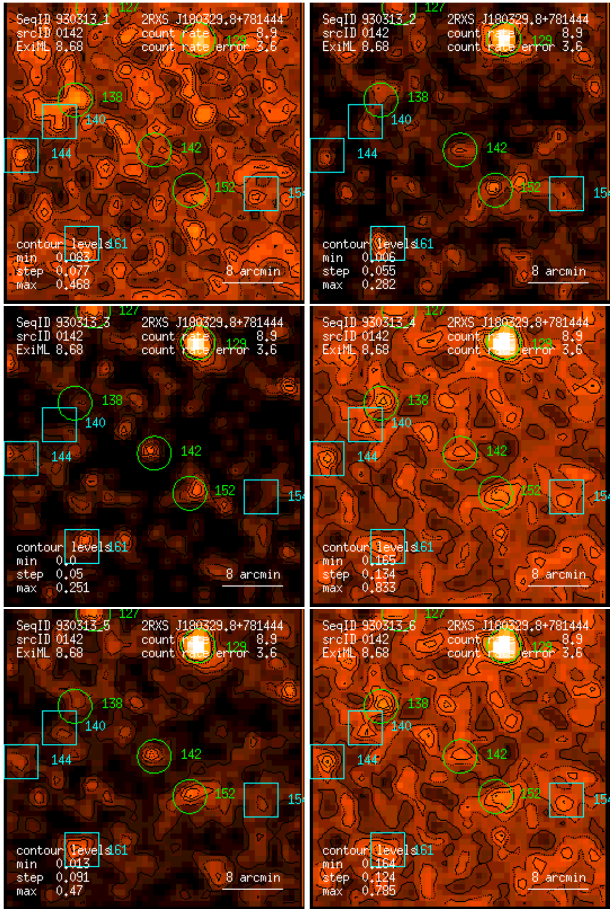
Figure 142: RASS 930313: detection 0142: band rate images, Gaussian filter: (1) PSPC channels 11 – 41, (2) 52 – 90, (3) 91 – 201, (4) 11 – 235, (5) 52 – 201, (6) 11 – 201. Broad band rates in counts/ks. Band rate contour levels in counts/ks/arcmin 2 .
