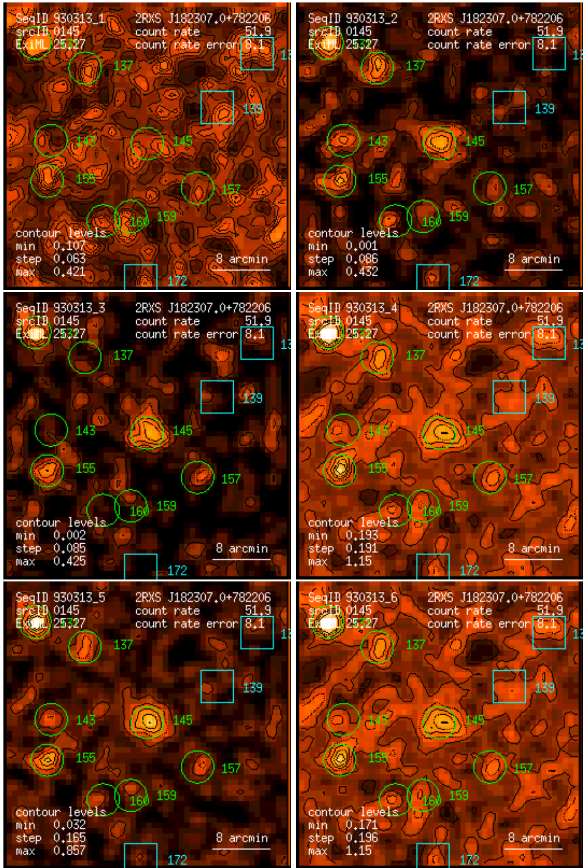
Figure 145: RASS 930313: detection 0145: band rate images, Gaussian filter: (1) PSPC channels 11 – 41, (2) 52 – 90, (3) 91 – 201, (4) 11 – 235, (5) 52 – 201, (6) 11 – 201. Broad band rates in counts/ks. Band rate contour levels in counts/ks/arcmin 2 .
