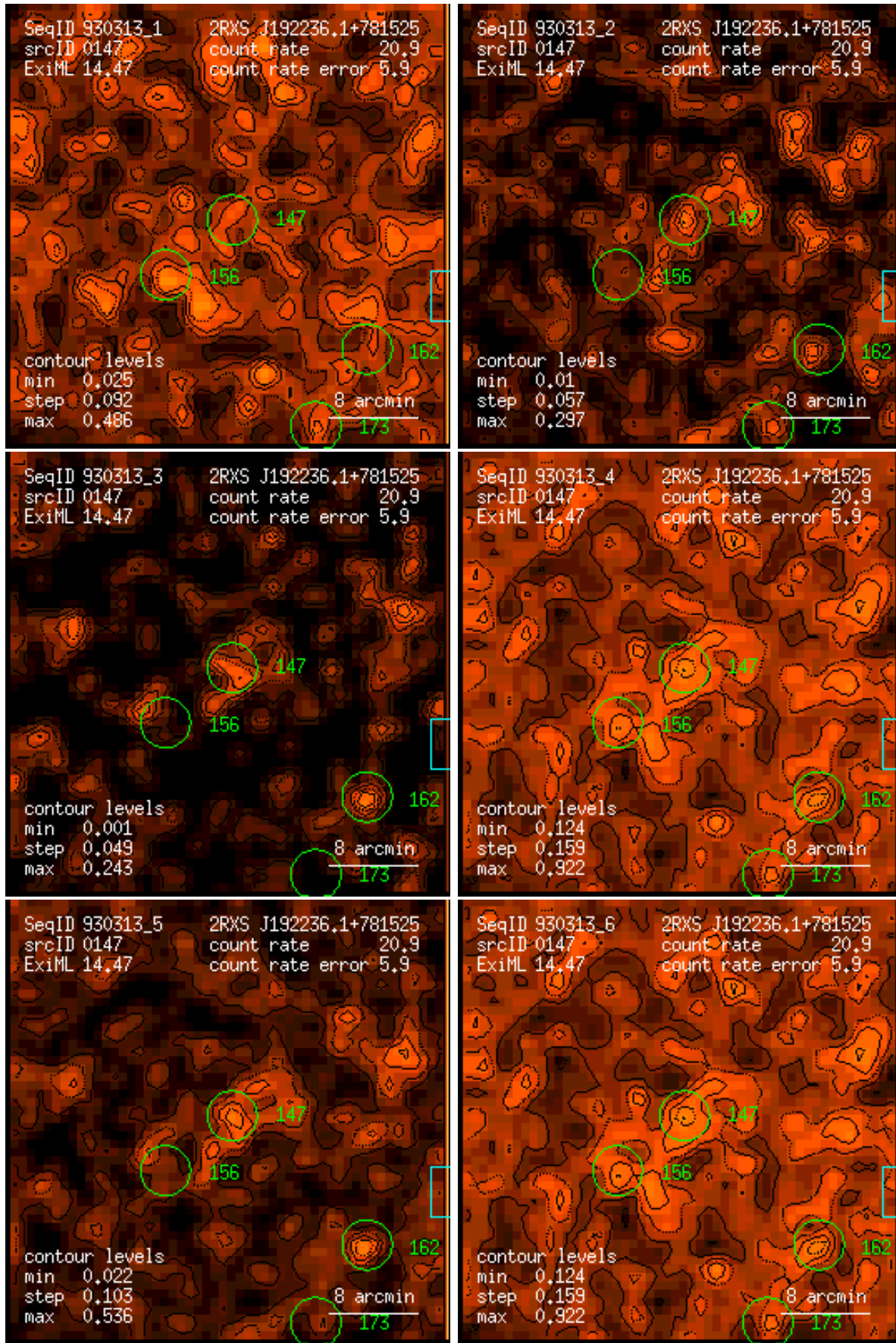
Figure 147: RASS 930313: detection 0147: band rate images, Gaussian filter: (1) PSPC channels 11 – 41, (2) 52 – 90, (3) 91 – 201, (4) 11 – 235, (5) 52 – 201, (6) 11 – 201. Broad band rates in counts/ks. Band rate contour levels in counts/ks/arcmin 2 .
