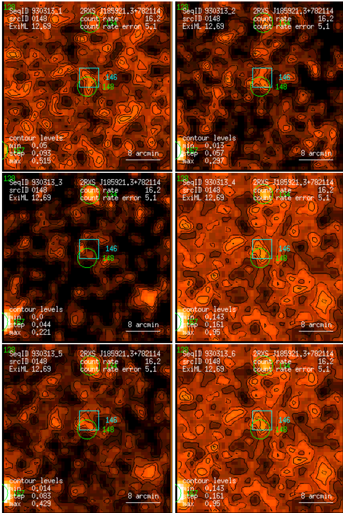
Figure 148: RASS 930313: detection 0148: band rate images, Gaussian filter: (1) PSPC channels 11 – 41, (2) 52 – 90, (3) 91 – 201, (4) 11 – 235, (5) 52 – 201, (6) 11 – 201. Broad band rates in counts/ks. Band rate contour levels in counts/ks/arcmin 2 .
