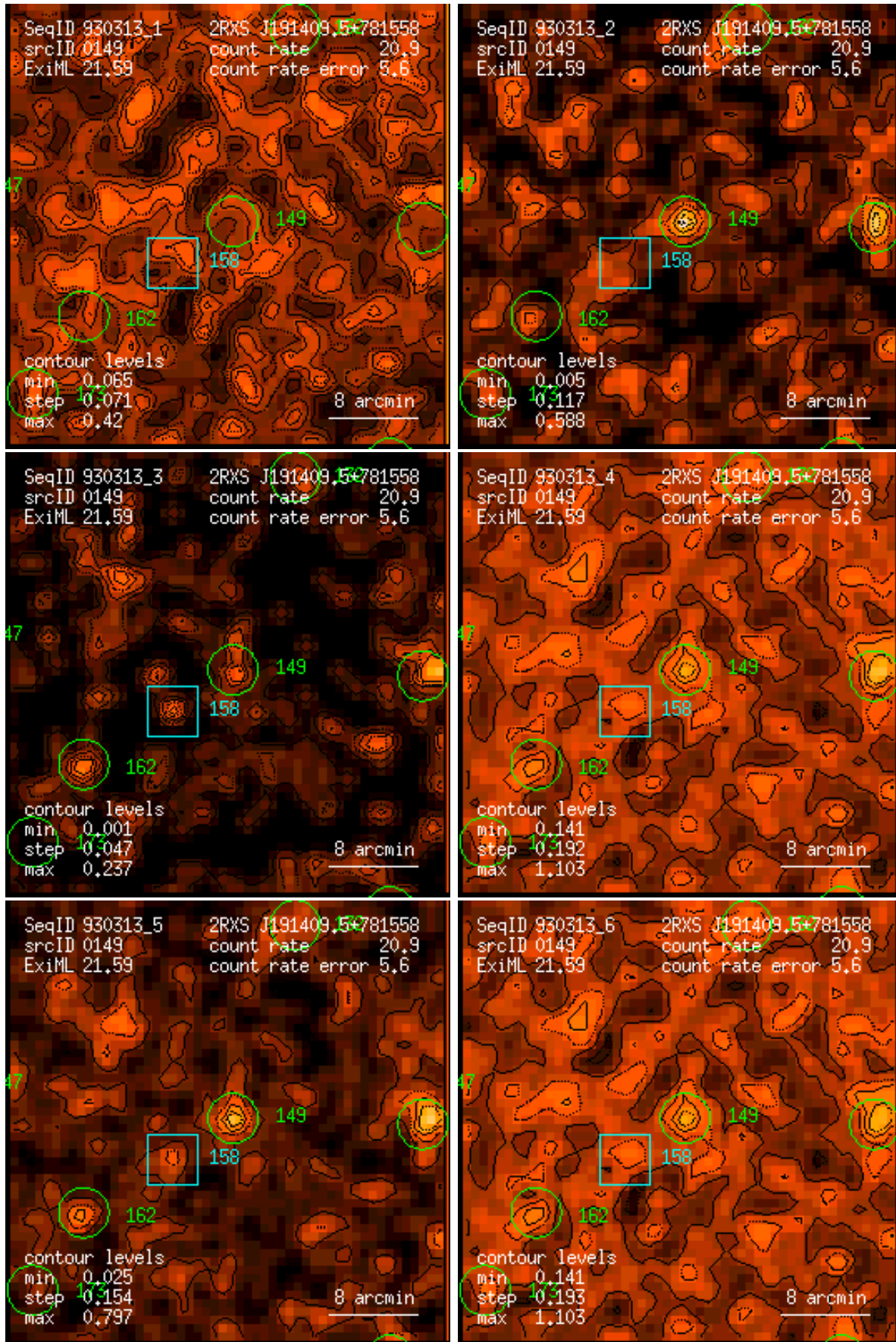
Figure 149: RASS 930313: detection 0149: band rate images, Gaussian filter: (1) PSPC channels 11 – 41, (2) 52 – 90, (3) 91 – 201, (4) 11 – 235, (5) 52 – 201, (6) 11 – 201. Broad band rates in counts/ks. Band rate contour levels in counts/ks/arcmin 2 .
