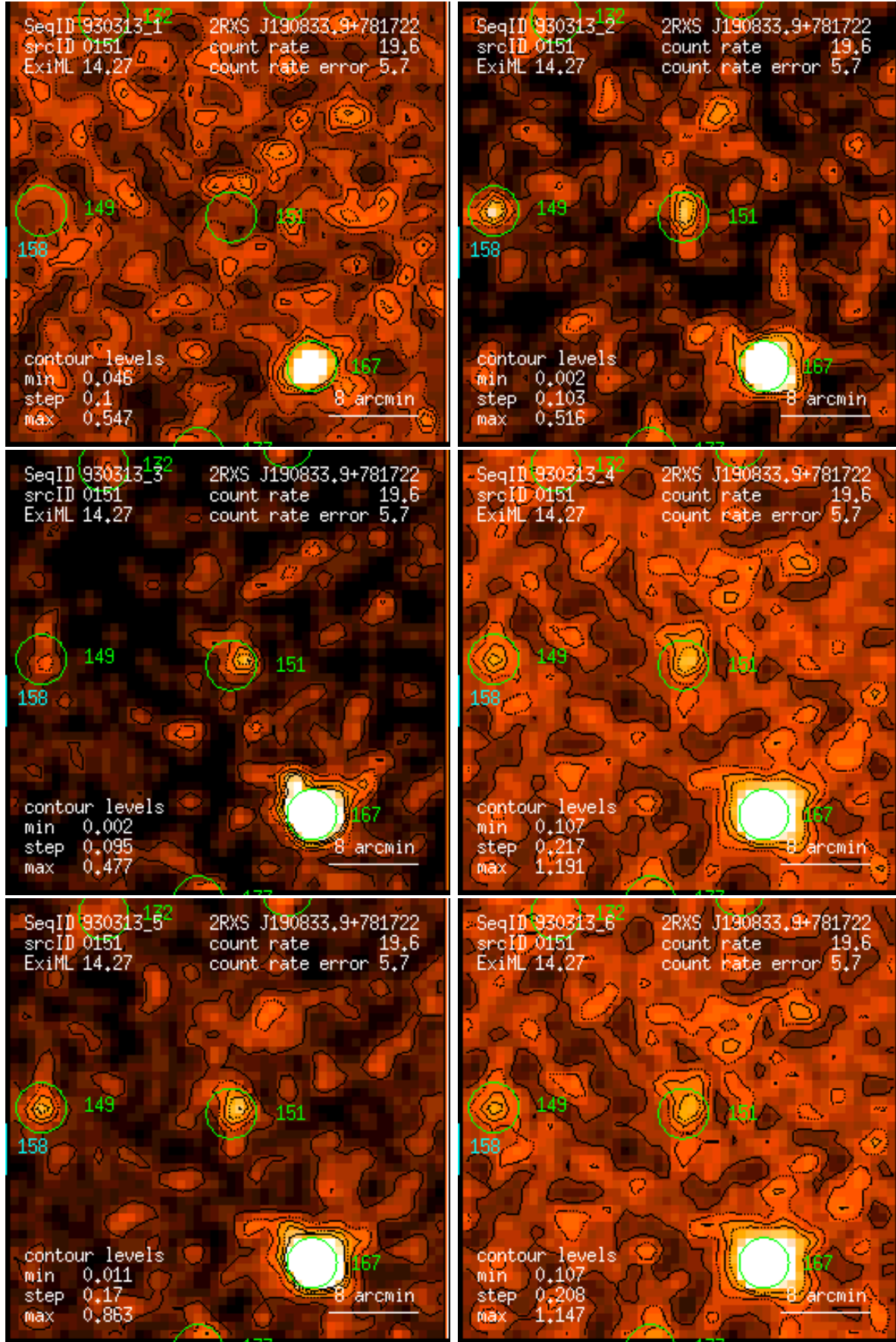
Figure 151: RASS 930313: detection 0151: band rate images, Gaussian filter: (1) PSPC channels 11 – 41, (2) 52 – 90, (3) 91 – 201, (4) 11 – 235, (5) 52 – 201, (6) 11 – 201. Broad band rates in counts/ks. Band rate contour levels in counts/ks/arcmin 2 .
