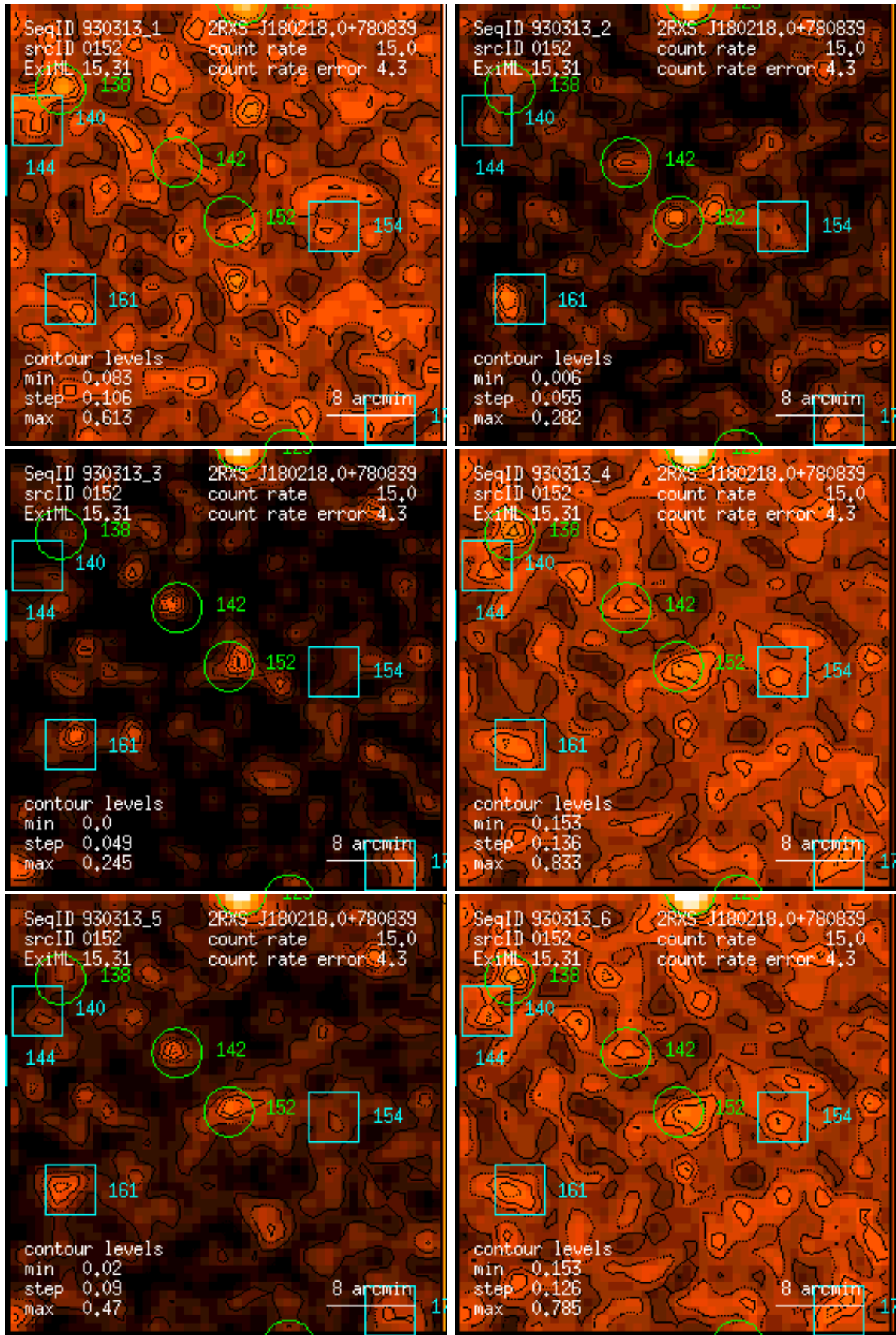
Figure 152: RASS 930313: detection 0152: band rate images, Gaussian filter: (1) PSPC channels 11 – 41, (2) 52 – 90, (3) 91 – 201, (4) 11 – 235, (5) 52 – 201, (6) 11 – 201. Broad band rates in counts/ks. Band rate contour levels in counts/ks/arcmin 2 .
