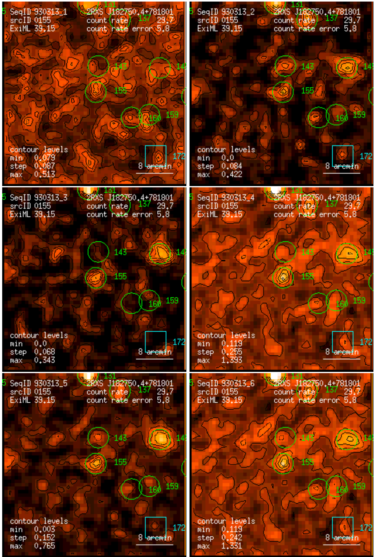
Figure 155: RASS 930313: detection 0155: band rate images, Gaussian filter: (1) PSPC channels 11 – 41, (2) 52 – 90, (3) 91 – 201, (4) 11 – 235, (5) 52 – 201, (6) 11 – 201. Broad band rates in counts/ks. Band rate contour levels in counts/ks/arcmin 2 .
