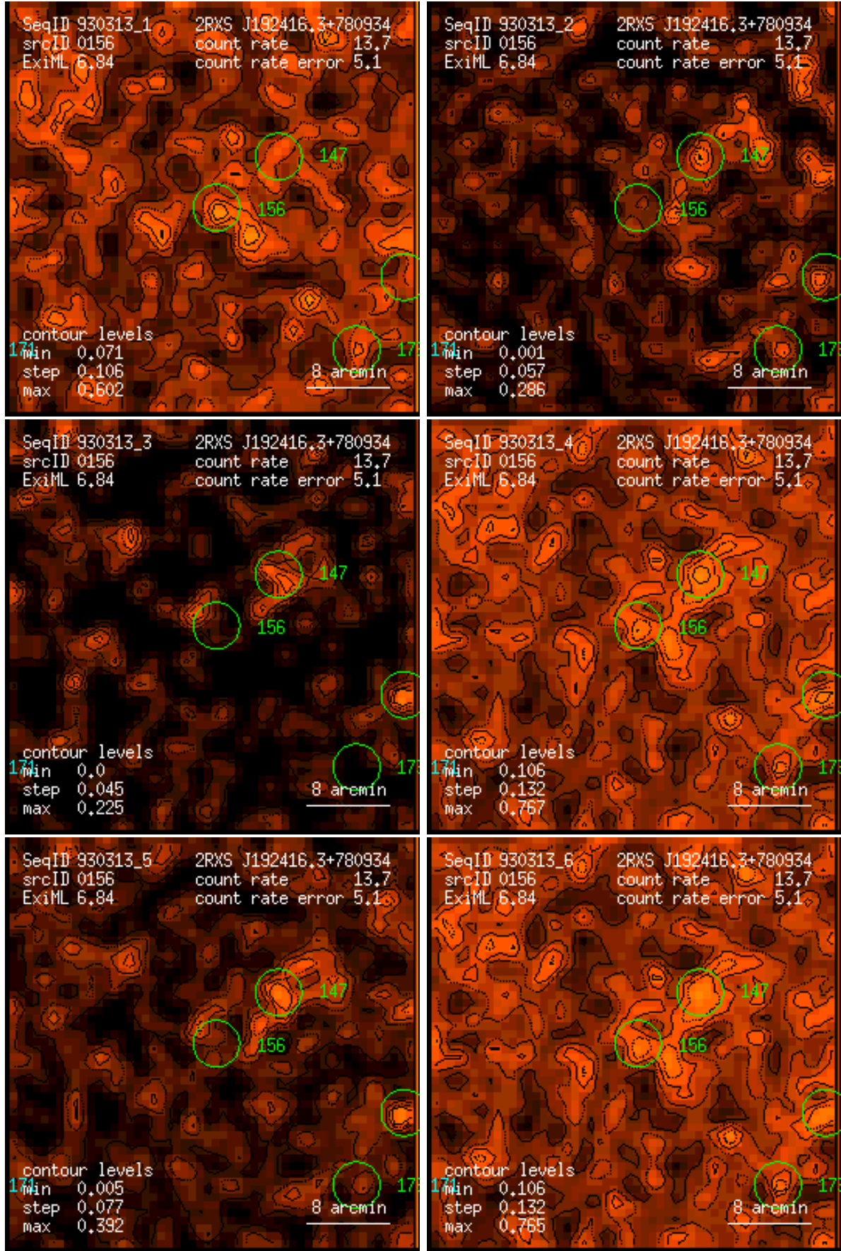
Figure 156: RASS 930313: detection 0156: band rate images, Gaussian filter: (1) PSPC channels 11 – 41, (2) 52 – 90, (3) 91 – 201, (4) 11 – 235, (5) 52 – 201, (6) 11 – 201. Broad band rates in counts/ks. Band rate contour levels in counts/ks/arcmin 2 .
