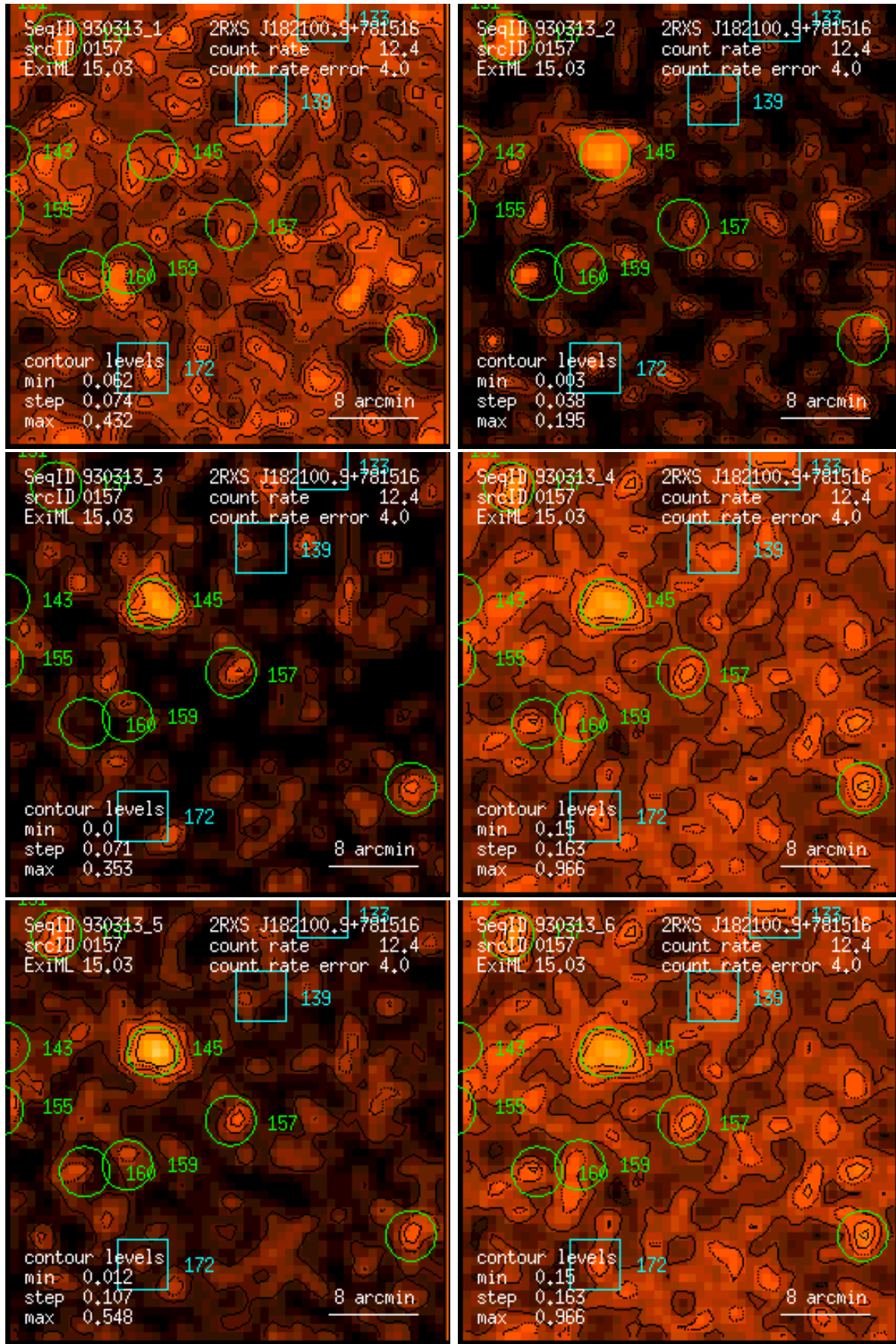
Figure 157: RASS 930313: detection 0157: band rate images, Gaussian filter: (1) PSPC channels 11 – 41, (2) 52 – 90, (3) 91 – 201, (4) 11 – 235, (5) 52 – 201, (6) 11 – 201. Broad band rates in counts/ks. Band rate contour levels in counts/ks/arcmin 2 .
