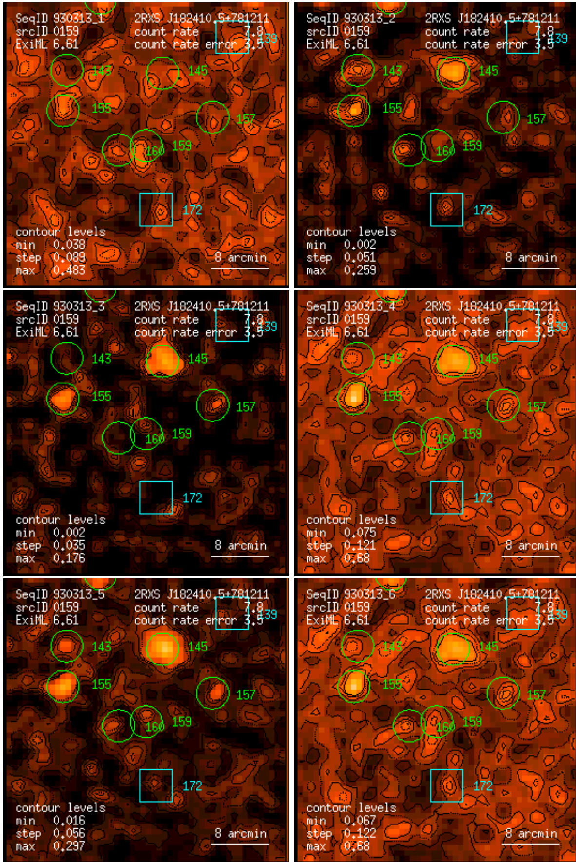
Figure 159: RASS 930313: detection 0159: band rate images, Gaussian filter: (1) PSPC channels 11 – 41, (2) 52 – 90, (3) 91 – 201, (4) 11 – 235, (5) 52 – 201, (6) 11 – 201. Broad band rates in counts/ks. Band rate contour levels in counts/ks/arcmin 2 .
