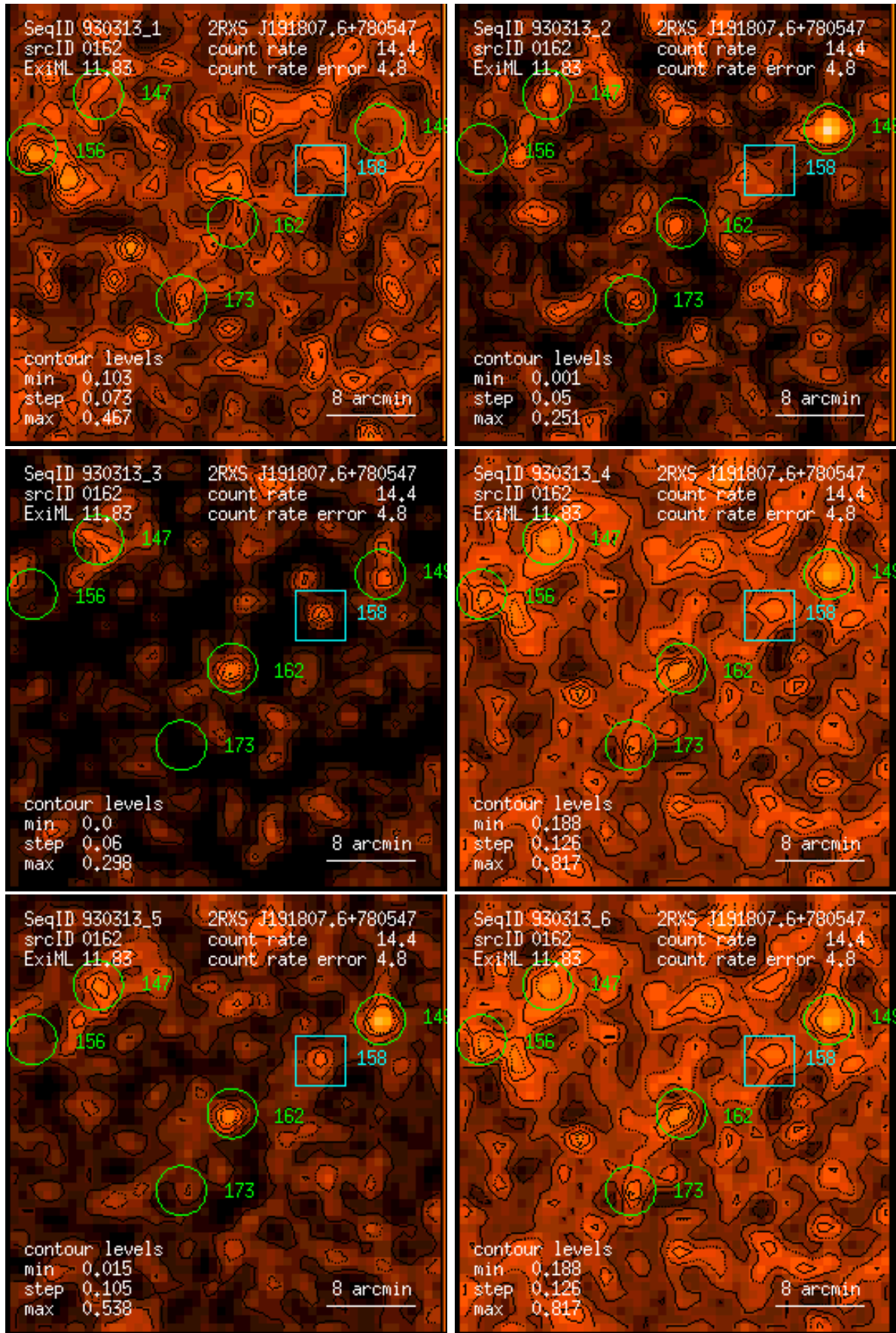
Figure 162: RASS 930313: detection 0162: band rate images, Gaussian filter: (1) PSPC channels 11 – 41, (2) 52 – 90, (3) 91 – 201, (4) 11 – 235, (5) 52 – 201, (6) 11 – 201. Broad band rates in counts/ks. Band rate contour levels in counts/ks/arcmin 2 .
