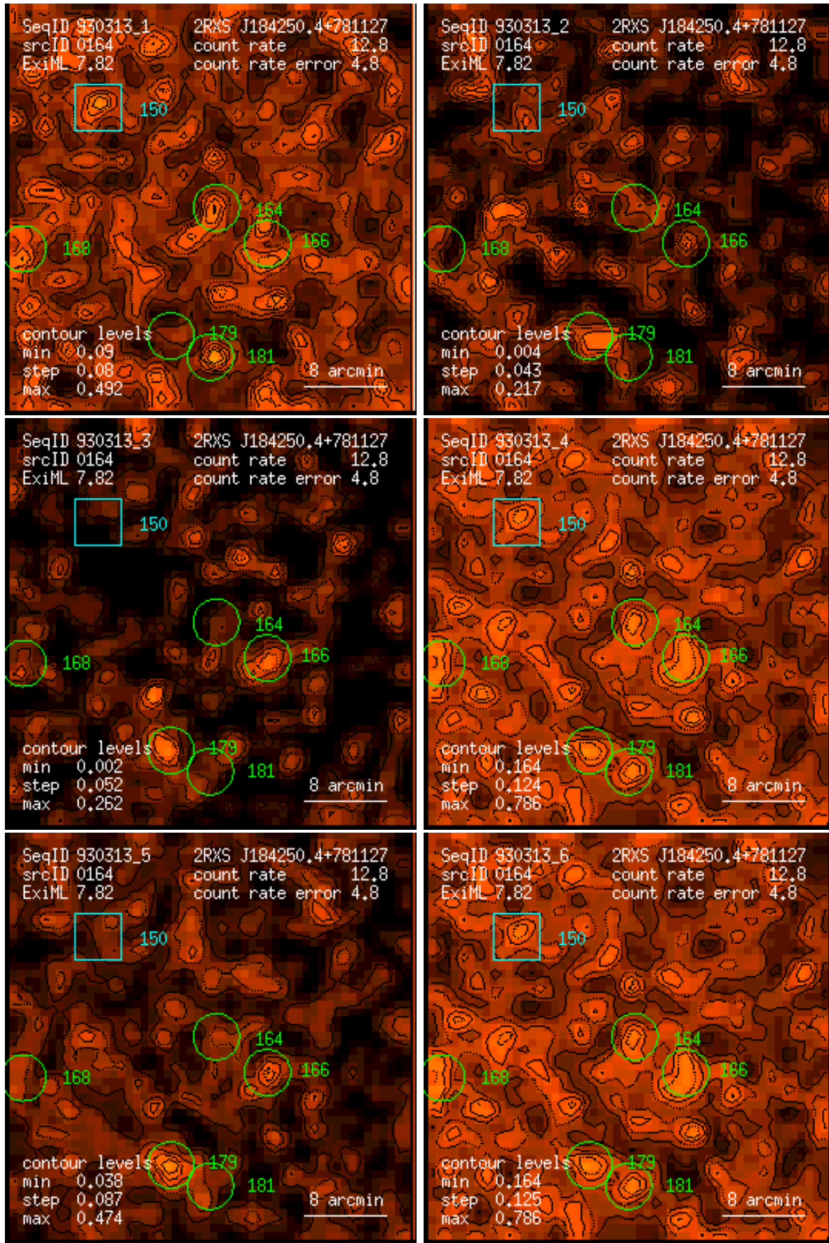
Figure 164: RASS 930313: detection 0164: band rate images, Gaussian filter: (1) PSPC channels 11 – 41, (2) 52 – 90, (3) 91 – 201, (4) 11 – 235, (5) 52 – 201, (6) 11 – 201. Broad band rates in counts/ks. Band rate contour levels in counts/ks/arcmin 2 .
