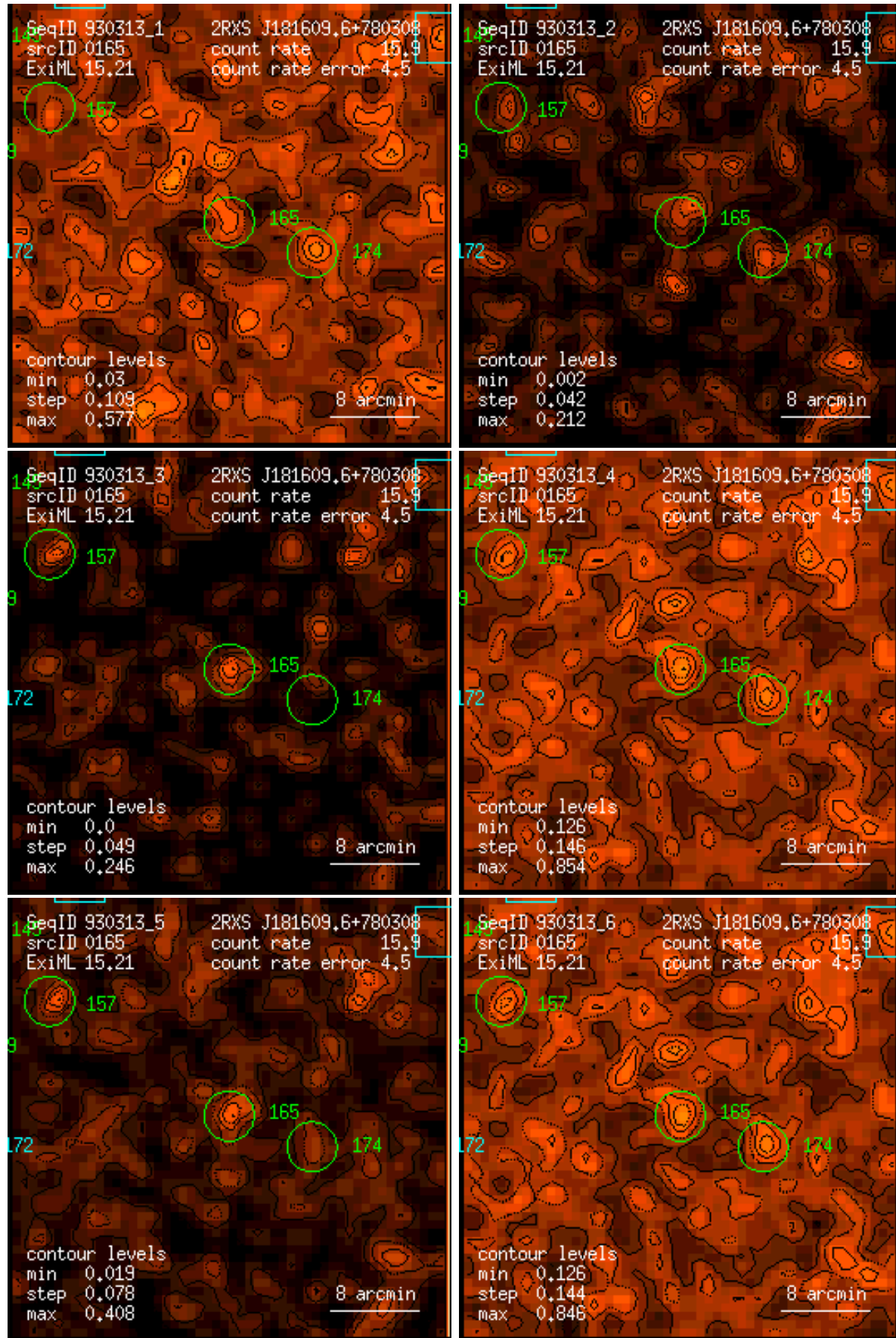
Figure 165: RASS 930313: detection 0165: band rate images, Gaussian filter: (1) PSPC channels 11 – 41, (2) 52 – 90, (3) 91 – 201, (4) 11 – 235, (5) 52 – 201, (6) 11 – 201. Broad band rates in counts/ks. Band rate contour levels in counts/ks/arcmin 2 .
