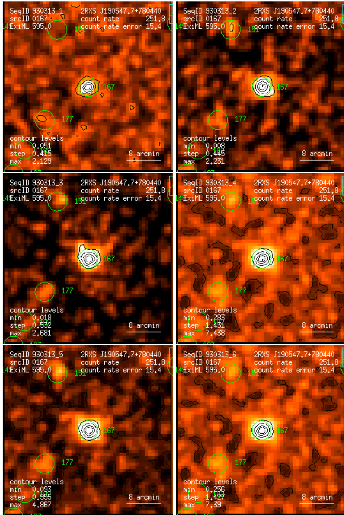
Figure 167: RASS 930313: detection 0167: band rate images, Gaussian filter: (1) PSPC channels 11 – 41, (2) 52 – 90, (3) 91 – 201, (4) 11 – 235, (5) 52 – 201, (6) 11 – 201. Broad band rates in counts/ks. Band rate contour levels in counts/ks/arcmin 2 .
