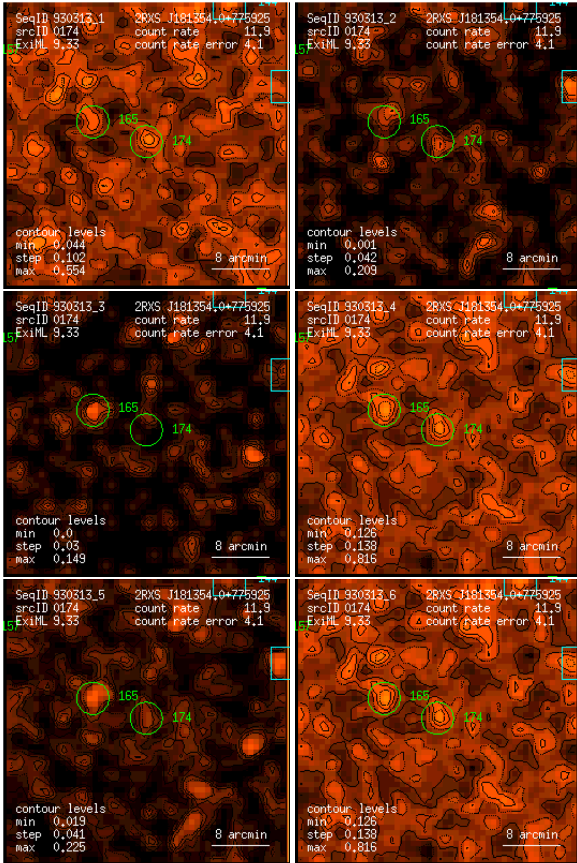
Figure 174: RASS 930313: detection 0174: band rate images, Gaussian filter: (1) PSPC channels 11 – 41, (2) 52 – 90, (3) 91 – 201, (4) 11 – 235, (5) 52 – 201, (6) 11 – 201. Broad band rates in counts/ks. Band rate contour levels in counts/ks/arcmin 2 .
