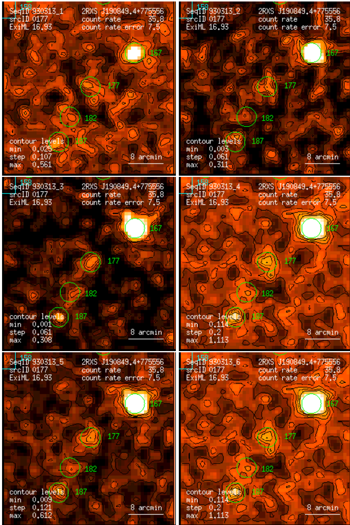
Figure 177: RASS 930313: detection 0177: band rate images, Gaussian filter: (1) PSPC channels 11 – 41, (2) 52 – 90, (3) 91 – 201, (4) 11 – 235, (5) 52 – 201, (6) 11 – 201. Broad band rates in counts/ks. Band rate contour levels in counts/ks/arcmin 2 .
