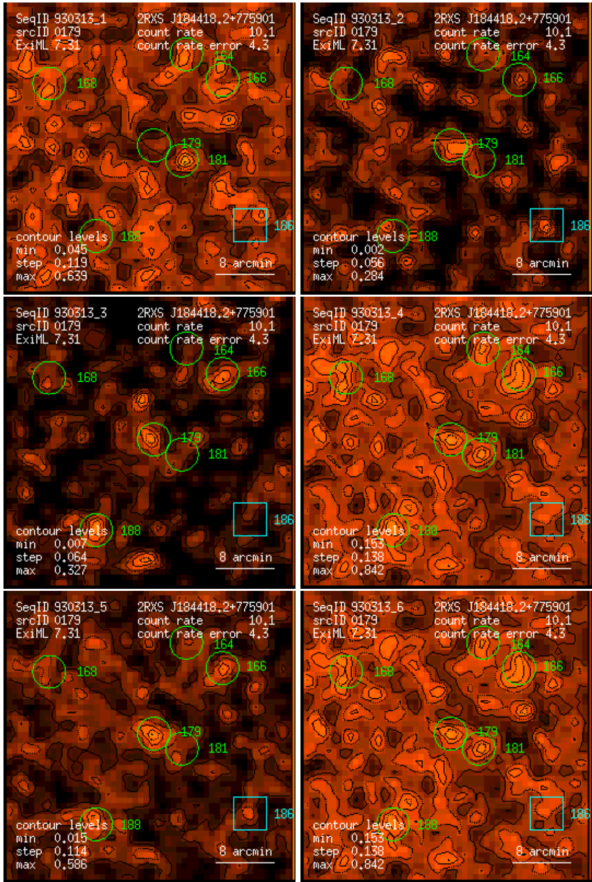
Figure 179: RASS 930313: detection 0179: band rate images, Gaussian filter: (1) PSPC channels 11 – 41, (2) 52 – 90, (3) 91 – 201, (4) 11 – 235, (5) 52 – 201, (6) 11 – 201. Broad band rates in counts/ks. Band rate contour levels in counts/ks/arcmin 2 .
