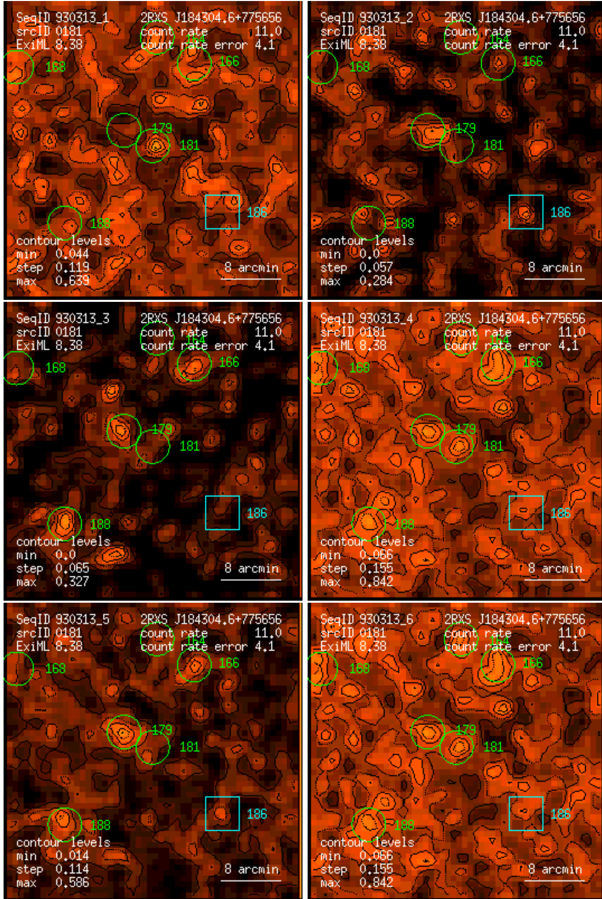
Figure 181: RASS 930313: detection 0181: band rate images, Gaussian filter: (1) PSPC channels 11 – 41, (2) 52 – 90, (3) 91 – 201, (4) 11 – 235, (5) 52 – 201, (6) 11 – 201. Broad band rates in counts/ks. Band rate contour levels in counts/ks/arcmin 2 .
