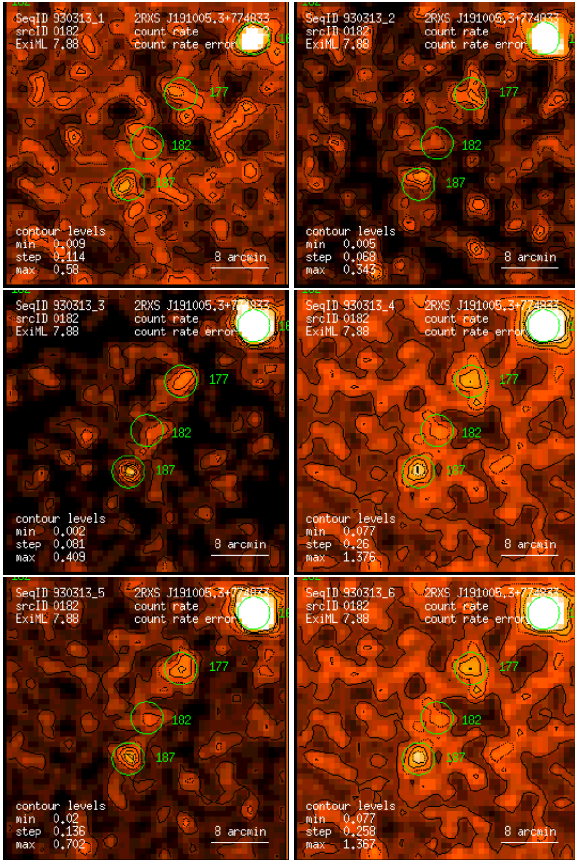
Figure 182: RASS 930313: detection 0182: band rate images, Gaussian filter: (1) PSPC channels 11 – 41, (2) 52 – 90, (3) 91 – 201, (4) 11 – 235, (5) 52 – 201, (6) 11 – 201. Broad band rates in counts/ks. Band rate contour levels in counts/ks/arcmin 2 .
