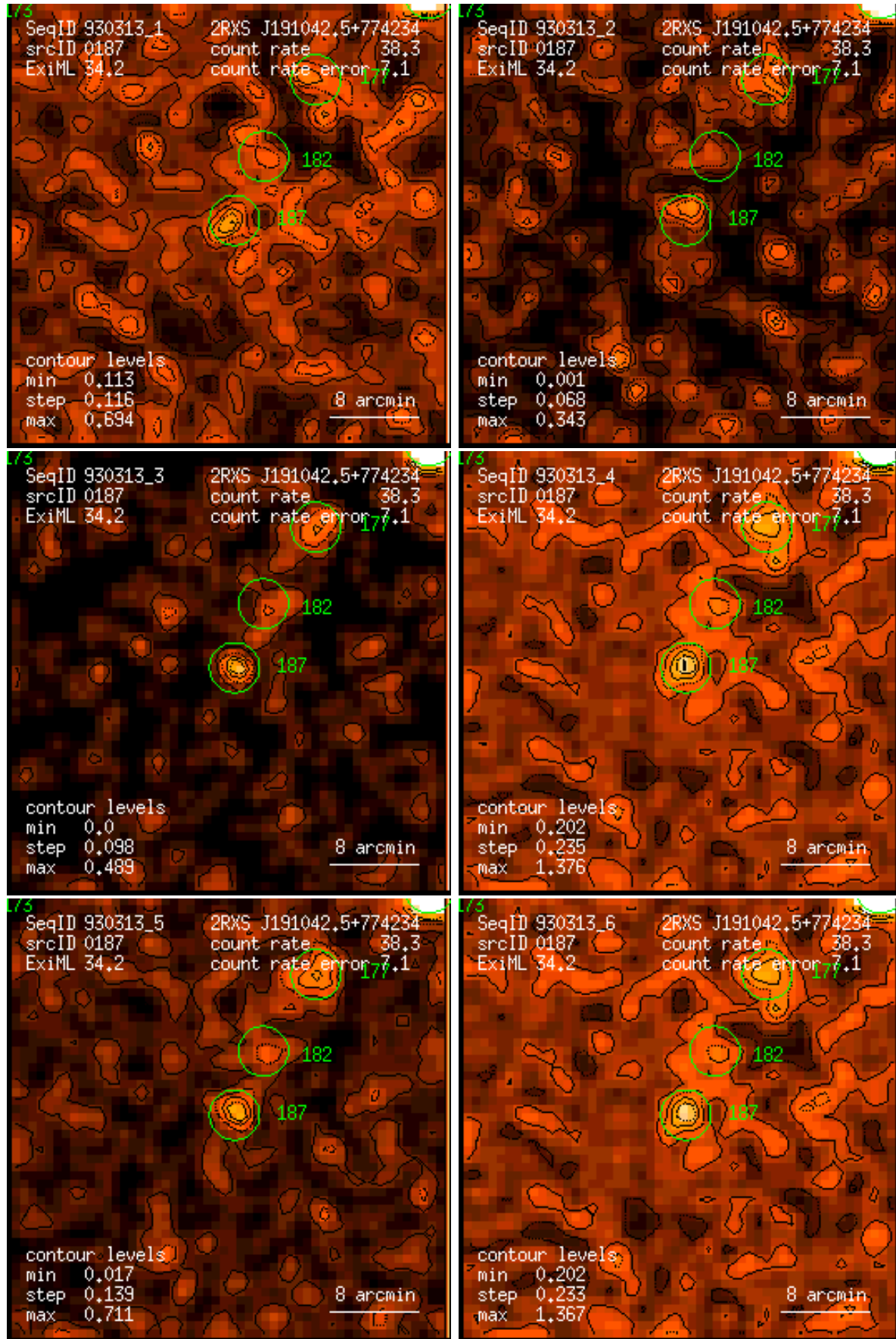
Figure 187: RASS 930313: detection 0187: band rate images, Gaussian filter: (1) PSPC channels 11 – 41, (2) 52 – 90, (3) 91 – 201, (4) 11 – 235, (5) 52 – 201, (6) 11 – 201. Broad band rates in counts/ks. Band rate contour levels in counts/ks/arcmin 2 .
