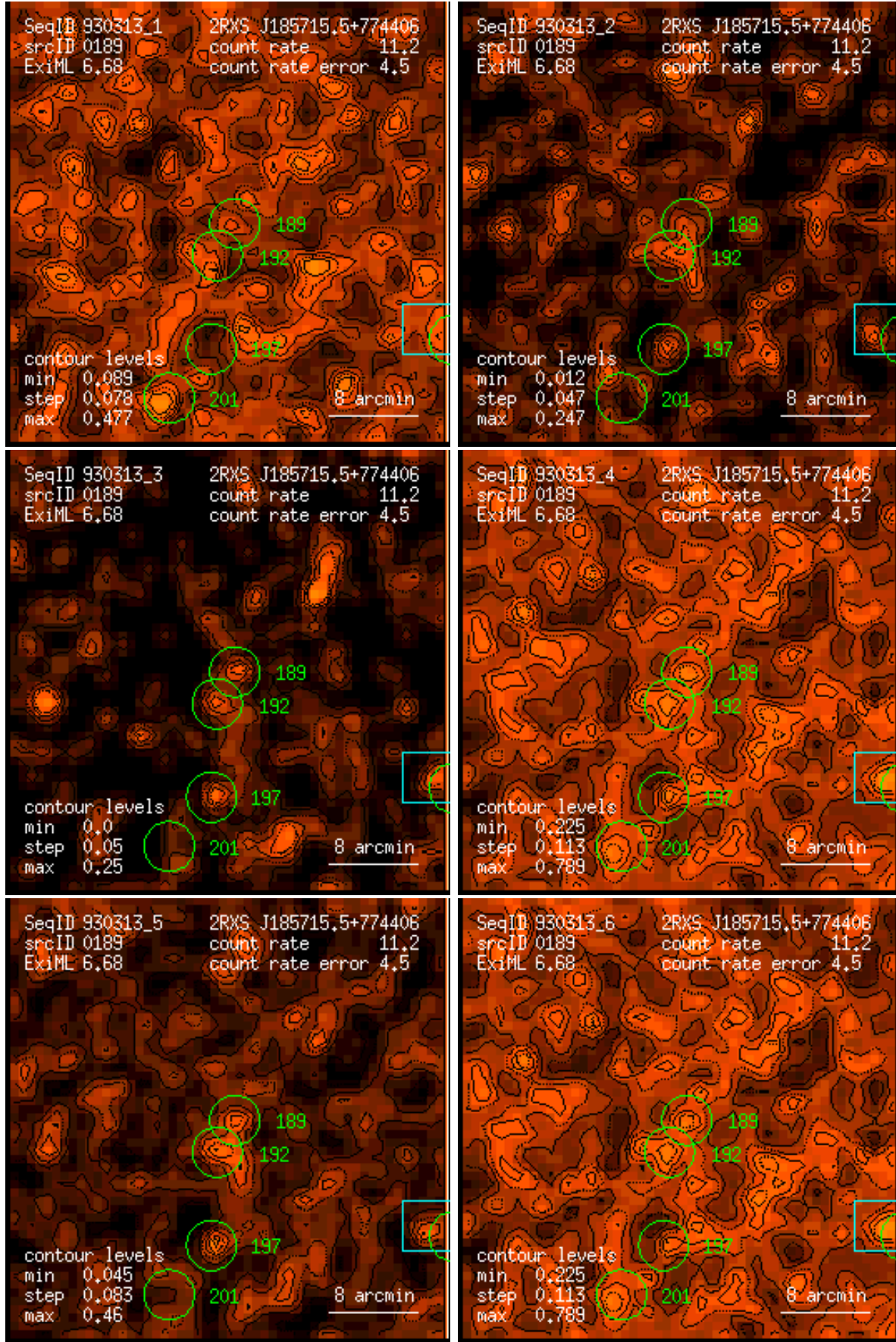
Figure 189: RASS 930313: detection 0189: band rate images, Gaussian filter: (1) PSPC channels 11 – 41, (2) 52 – 90, (3) 91 – 201, (4) 11 – 235, (5) 52 – 201, (6) 11 – 201. Broad band rates in counts/ks. Band rate contour levels in counts/ks/arcmin 2 .
