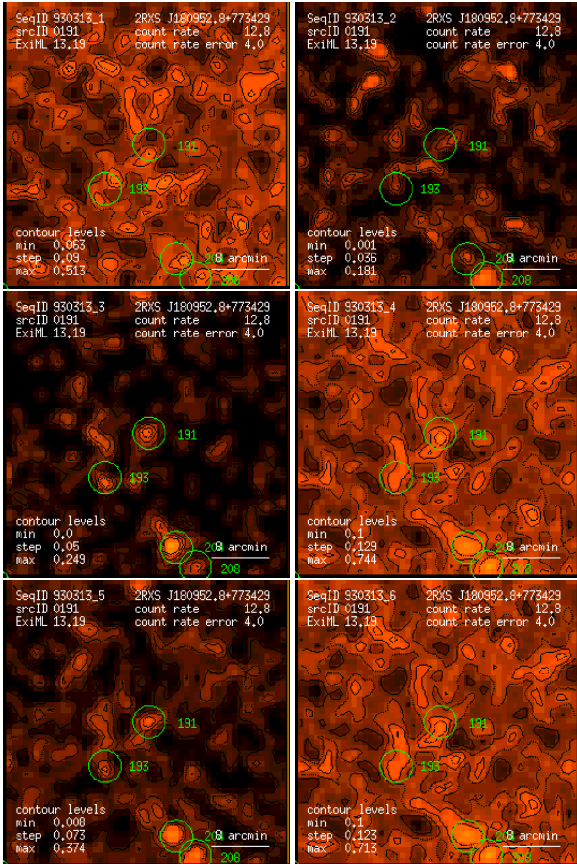
Figure 191: RASS 930313: detection 0191: band rate images, Gaussian filter: (1) PSPC channels 11 – 41, (2) 52 – 90, (3) 91 – 201, (4) 11 – 235, (5) 52 – 201, (6) 11 – 201. Broad band rates in counts/ks. Band rate contour levels in counts/ks/arcmin 2 .
