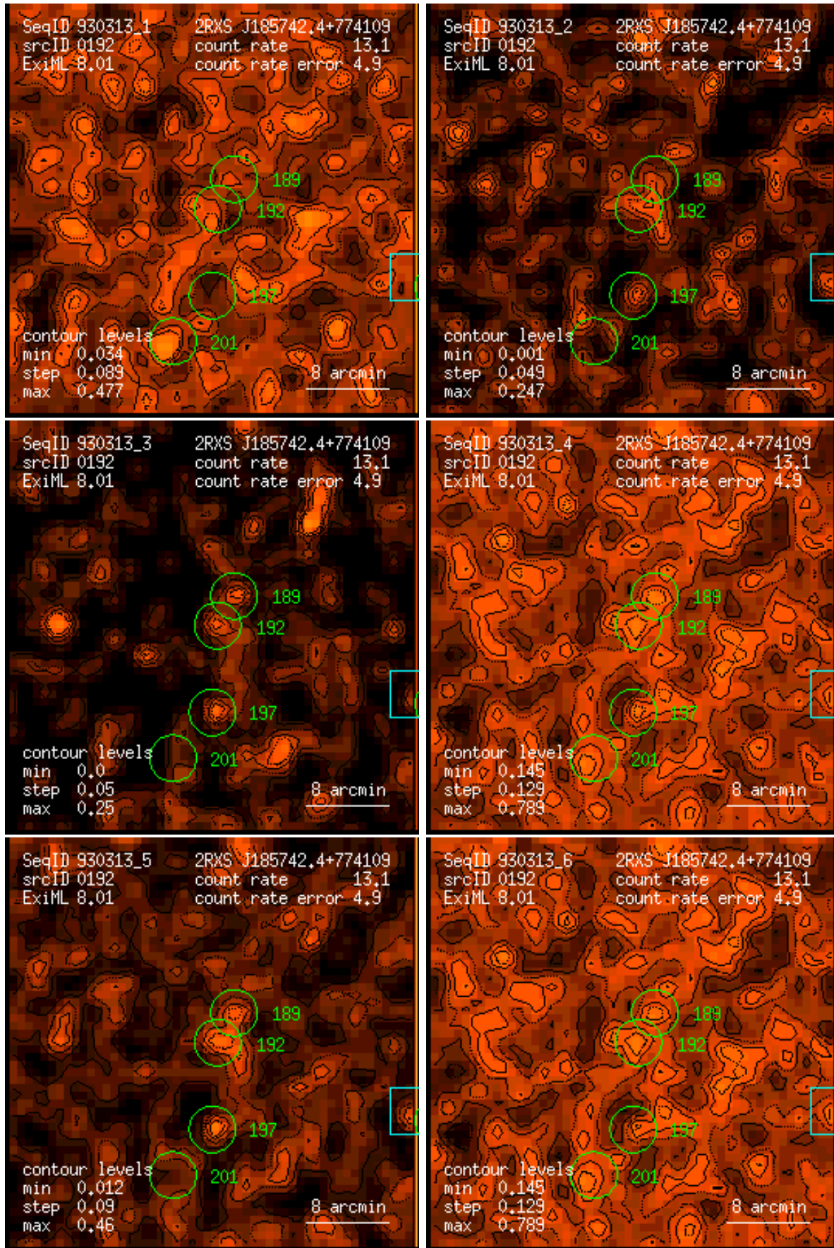
Figure 192: RASS 930313: detection 0192: band rate images, Gaussian filter: (1) PSPC channels 11 – 41, (2) 52 – 90, (3) 91 – 201, (4) 11 – 235, (5) 52 – 201, (6) 11 – 201. Broad band rates in counts/ks. Band rate contour levels in counts/ks/arcmin 2 .
