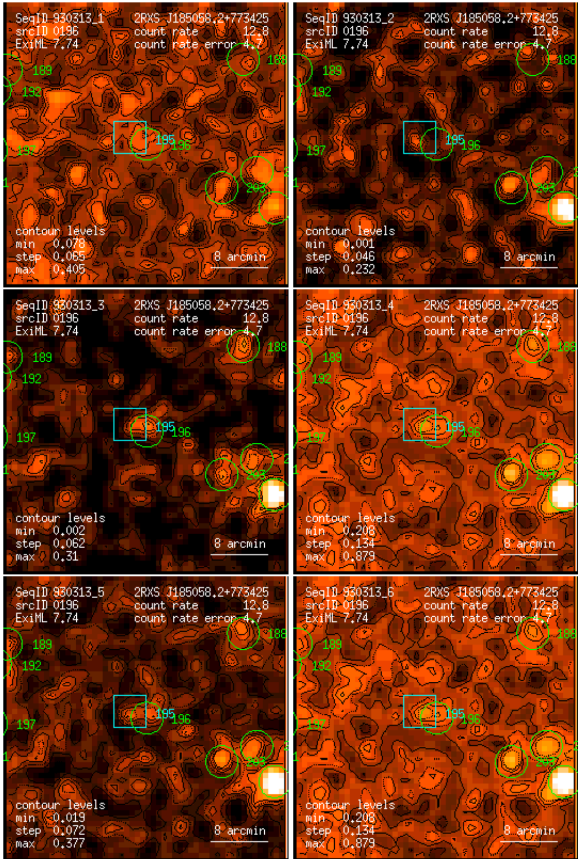
Figure 196: RASS 930313: detection 0196: band rate images, Gaussian filter: (1) PSPC channels 11 – 41, (2) 52 – 90, (3) 91 – 201, (4) 11 – 235, (5) 52 – 201, (6) 11 – 201. Broad band rates in counts/ks. Band rate contour levels in counts/ks/arcmin 2 .
