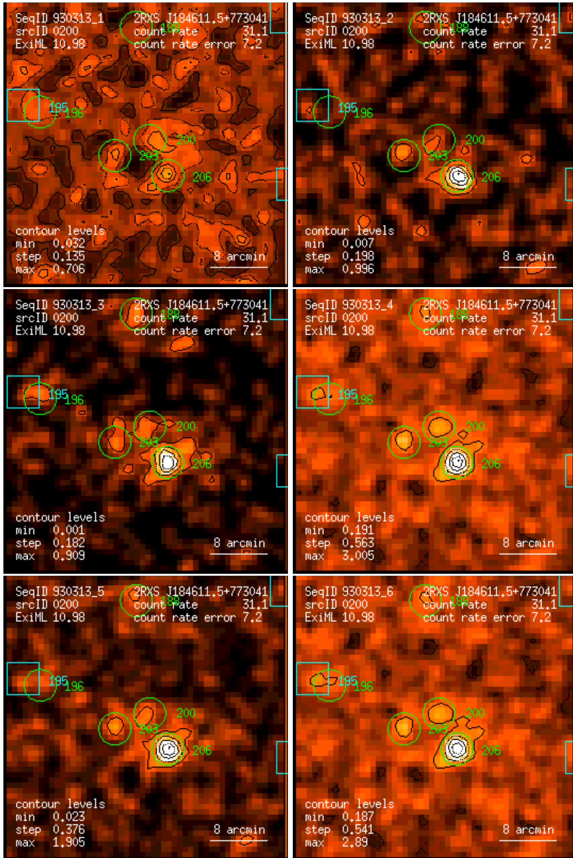
Figure 200: RASS 930313: detection 0200: band rate images, Gaussian filter: (1) PSPC channels 11 – 41, (2) 52 – 90, (3) 91 – 201, (4) 11 – 235, (5) 52 – 201, (6) 11 – 201. Broad band rates in counts/ks. Band rate contour levels in counts/ks/arcmin 2 .
