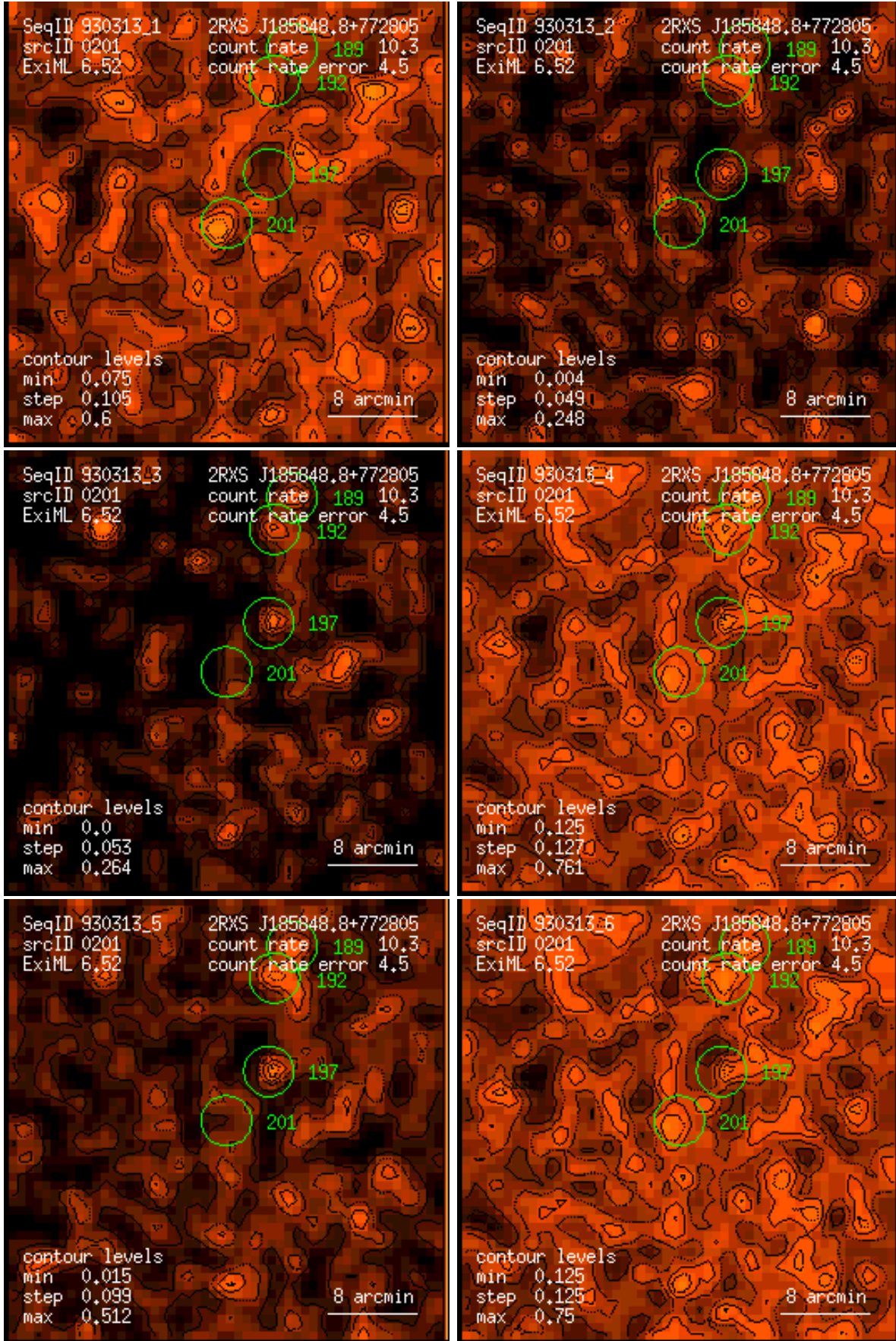
Figure 201: RASS 930313: detection 0201: band rate images, Gaussian filter: (1) PSPC channels 11 – 41, (2) 52 – 90, (3) 91 – 201, (4) 11 – 235, (5) 52 – 201, (6) 11 – 201. Broad band rates in counts/ks. Band rate contour levels in counts/ks/arcmin 2 .
