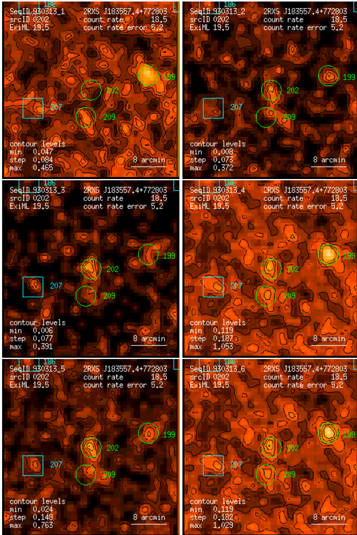
Figure 202: RASS 930313: detection 0202: band rate images, Gaussian filter: (1) PSPC channels 11 – 41, (2) 52 – 90, (3) 91 – 201, (4) 11 – 235, (5) 52 – 201, (6) 11 – 201. Broad band rates in counts/ks. Band rate contour levels in counts/ks/arcmin 2 .
