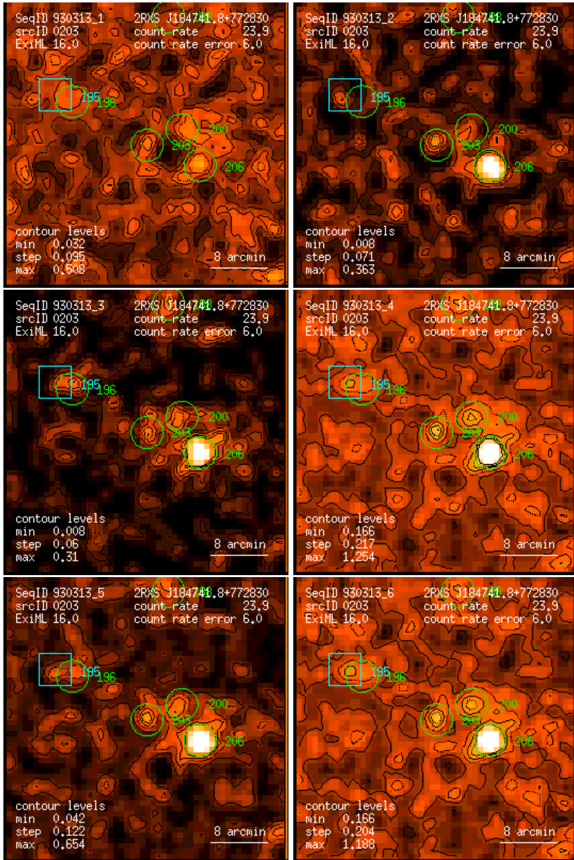
Figure 203: RASS 930313: detection 0203: band rate images, Gaussian filter: (1) PSPC channels 11 – 41, (2) 52 – 90, (3) 91 – 201, (4) 11 – 235, (5) 52 – 201, (6) 11 – 201. Broad band rates in counts/ks. Band rate contour levels in counts/ks/arcmin 2 .
