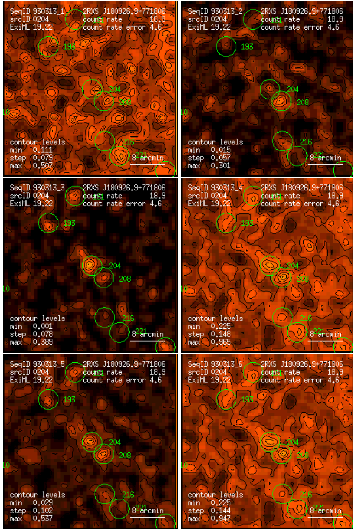
Figure 204: RASS 930313: detection 0204: band rate images, Gaussian filter: (1) PSPC channels 11 – 41, (2) 52 – 90, (3) 91 – 201, (4) 11 – 235, (5) 52 – 201, (6) 11 – 201. Broad band rates in counts/ks. Band rate contour levels in counts/ks/arcmin 2 .
