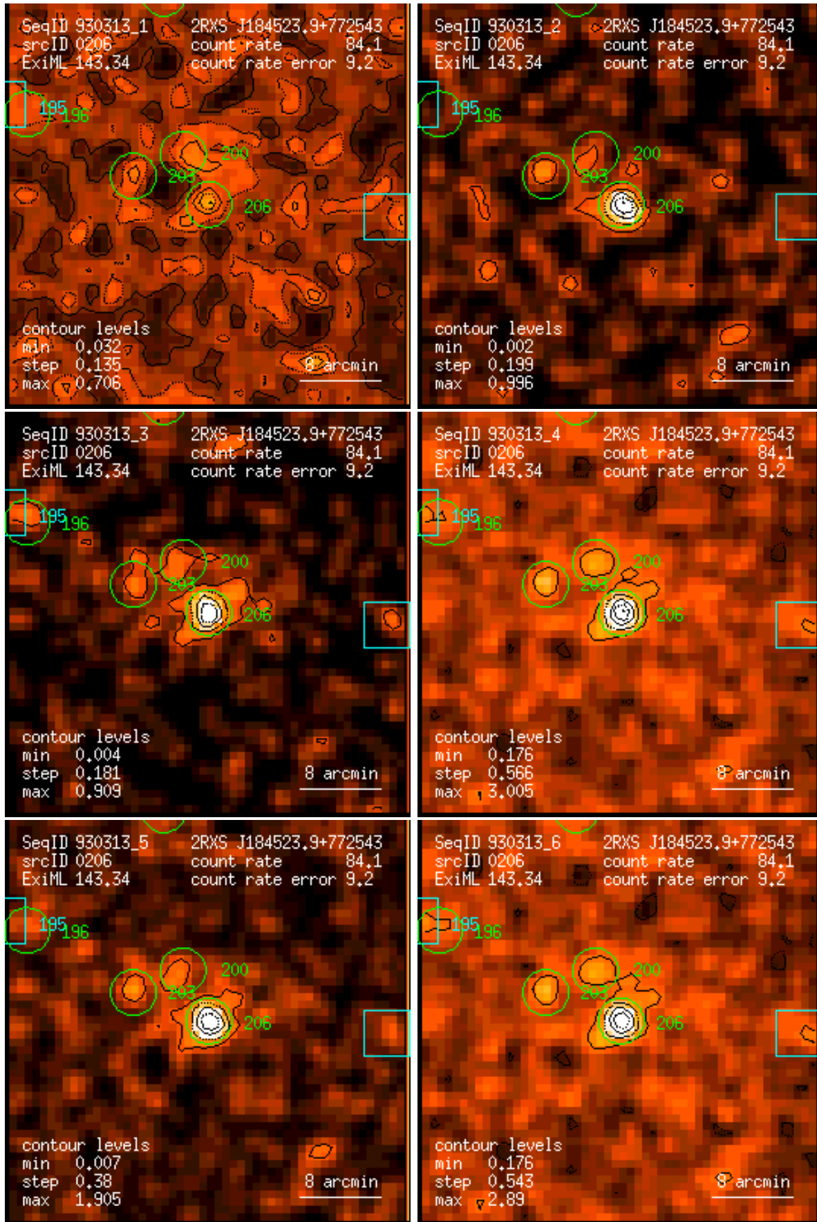
Figure 206: RASS 930313: detection 0206: band rate images, Gaussian filter: (1) PSPC channels 11 – 41, (2) 52 – 90, (3) 91 – 201, (4) 11 – 235, (5) 52 – 201, (6) 11 – 201. Broad band rates in counts/ks. Band rate contour levels in counts/ks/arcmin 2 .
