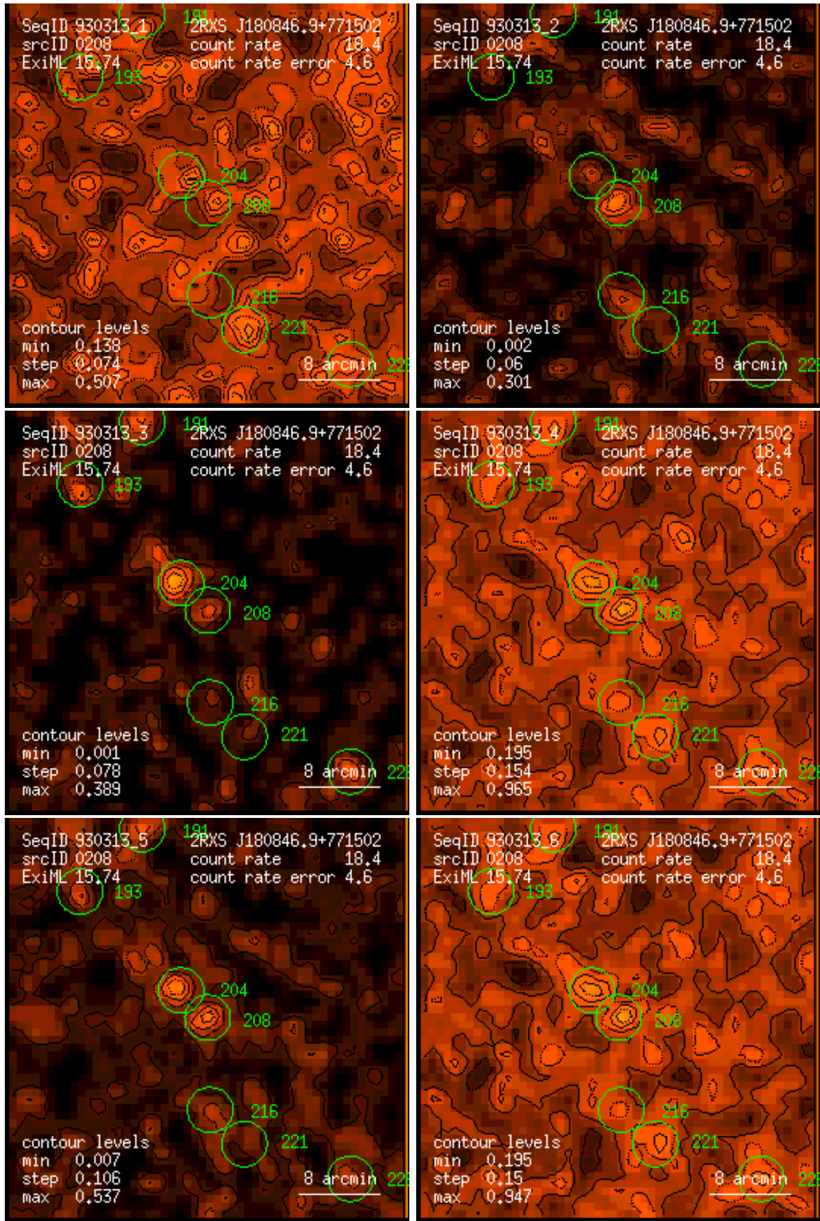
Figure 208: RASS 930313: detection 0208: band rate images, Gaussian filter: (1) PSPC channels 11 – 41, (2) 52 – 90, (3) 91 – 201, (4) 11 – 235, (5) 52 – 201, (6) 11 – 201. Broad band rates in counts/ks. Band rate contour levels in counts/ks/arcmin 2 .
