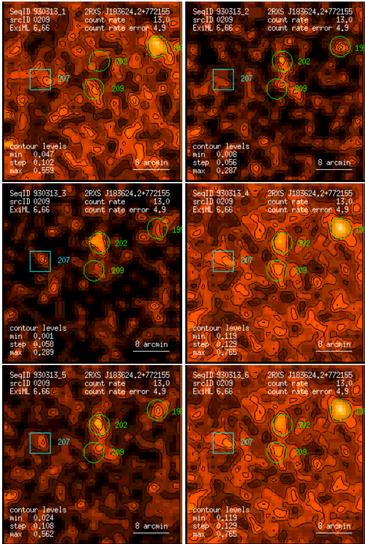
Figure 209: RASS 930313: detection 0209: band rate images, Gaussian filter: (1) PSPC channels 11 – 41, (2) 52 – 90, (3) 91 – 201, (4) 11 – 235, (5) 52 – 201, (6) 11 – 201. Broad band rates in counts/ks. Band rate contour levels in counts/ks/arcmin 2 .
