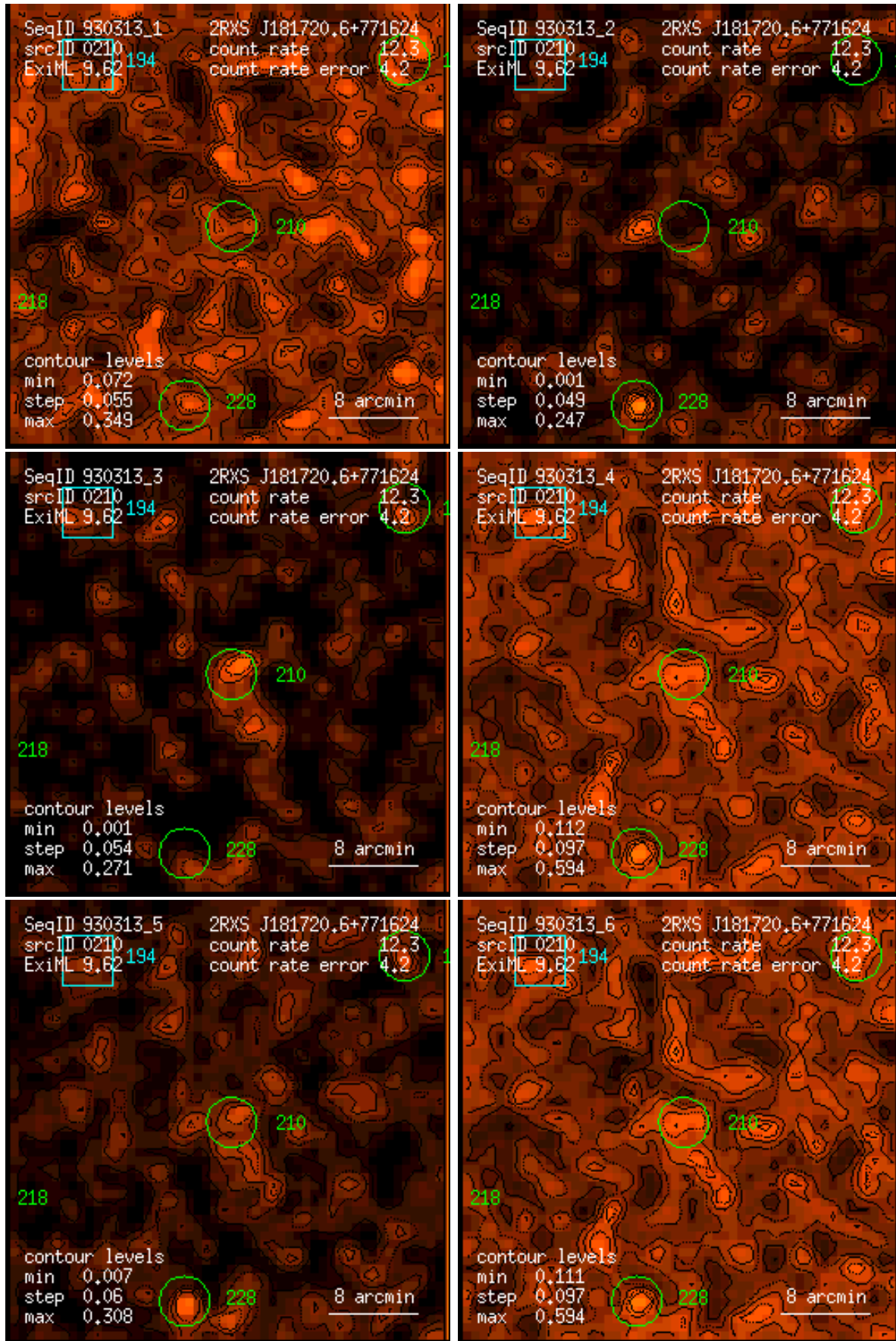
Figure 210: RASS 930313: detection 0210: band rate images, Gaussian filter: (1) PSPC channels 11 – 41, (2) 52 – 90, (3) 91 – 201, (4) 11 – 235, (5) 52 – 201, (6) 11 – 201. Broad band rates in counts/ks. Band rate contour levels in counts/ks/arcmin 2 .
