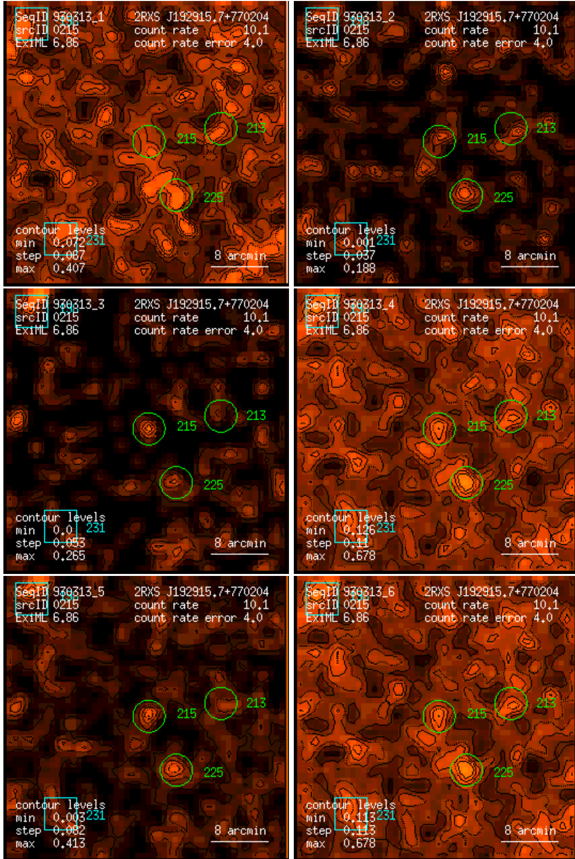
Figure 215: RASS 930313: detection 0215: band rate images, Gaussian filter: (1) PSPC channels 11 – 41, (2) 52 – 90, (3) 91 – 201, (4) 11 – 235, (5) 52 – 201, (6) 11 – 201. Broad band rates in counts/ks. Band rate contour levels in counts/ks/arcmin 2 .
