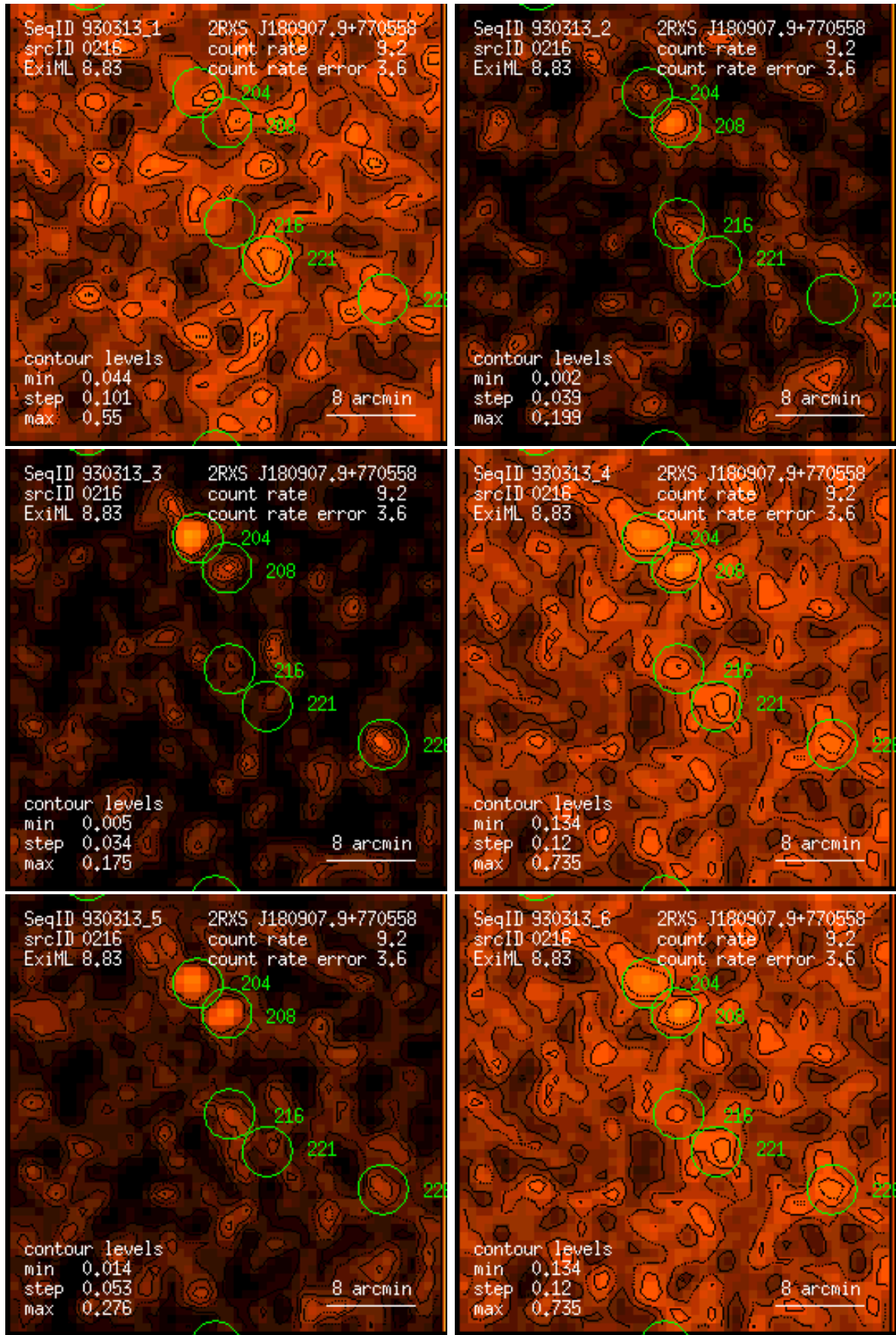
Figure 216: RASS 930313: detection 0216: band rate images, Gaussian filter: (1) PSPC channels 11 – 41, (2) 52 – 90, (3) 91 – 201, (4) 11 – 235, (5) 52 – 201, (6) 11 – 201. Broad band rates in counts/ks. Band rate contour levels in counts/ks/arcmin 2 .
