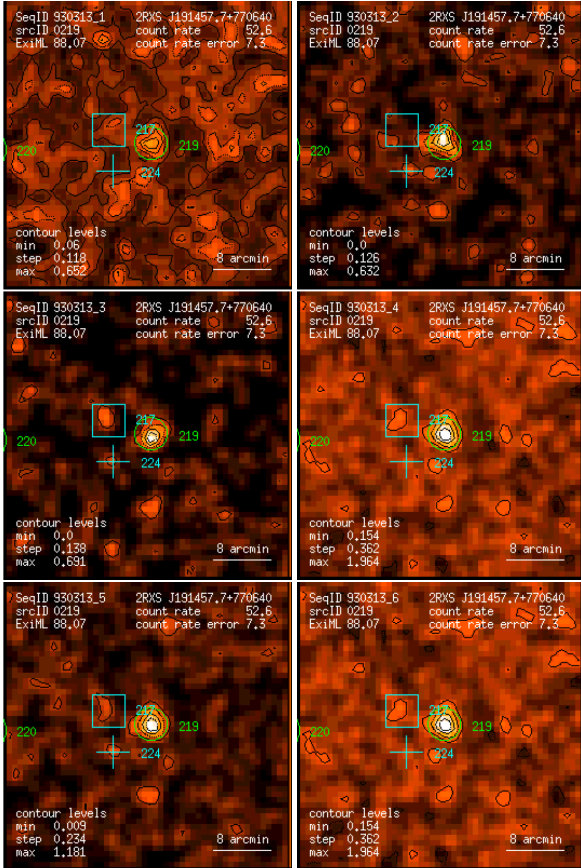
Figure 219: RASS 930313: detection 0219: band rate images, Gaussian filter: (1) PSPC channels 11 – 41, (2) 52 – 90, (3) 91 – 201, (4) 11 – 235, (5) 52 – 201, (6) 11 – 201. Broad band rates in counts/ks. Band rate contour levels in counts/ks/arcmin 2 .
