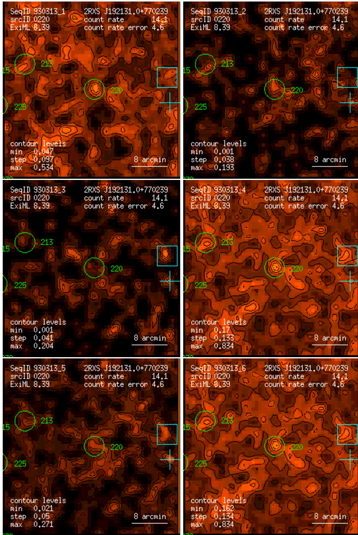
Figure 220: RASS 930313: detection 0220: band rate images, Gaussian filter: (1) PSPC channels 11 – 41, (2) 52 – 90, (3) 91 – 201, (4) 11 – 235, (5) 52 – 201, (6) 11 – 201. Broad band rates in counts/ks. Band rate contour levels in counts/ks/arcmin 2 .
