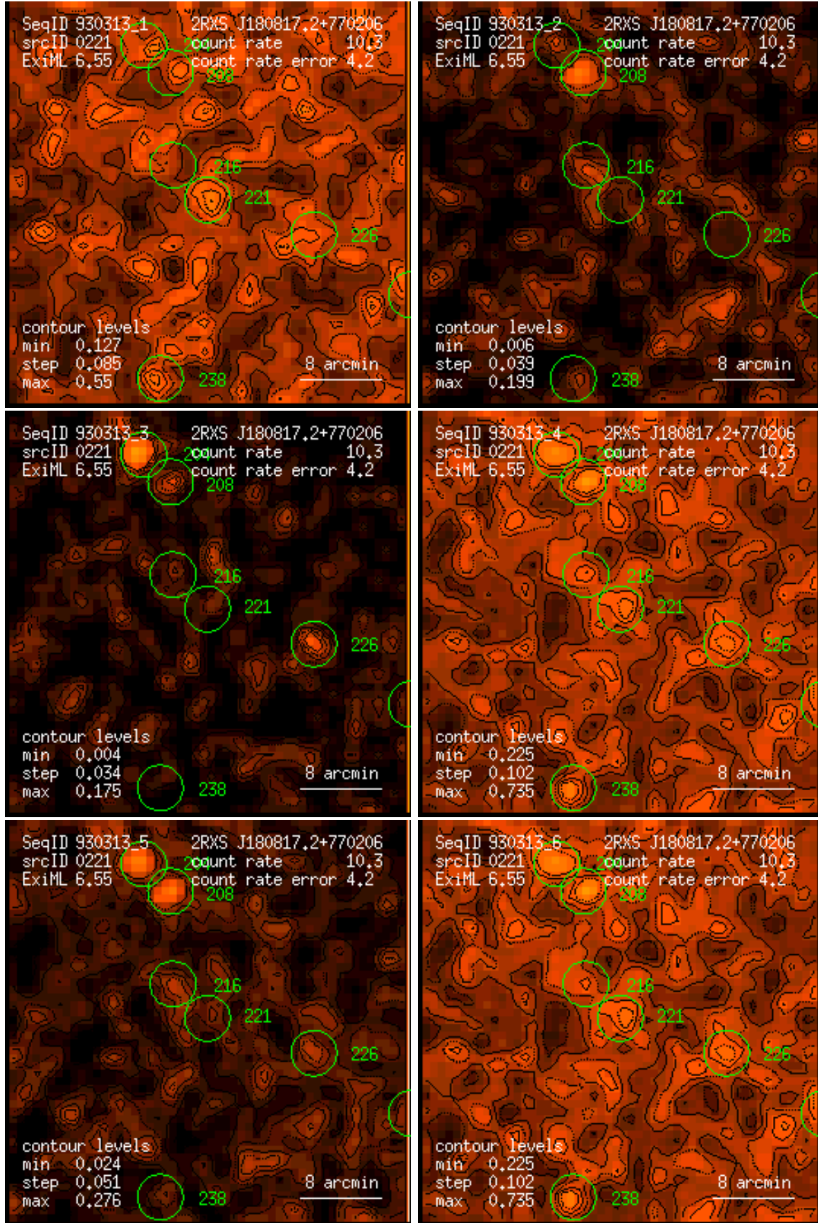
Figure 221: RASS 930313: detection 0221: band rate images, Gaussian filter: (1) PSPC channels 11 – 41, (2) 52 – 90, (3) 91 – 201, (4) 11 – 235, (5) 52 – 201, (6) 11 – 201. Broad band rates in counts/ks. Band rate contour levels in counts/ks/arcmin 2 .
