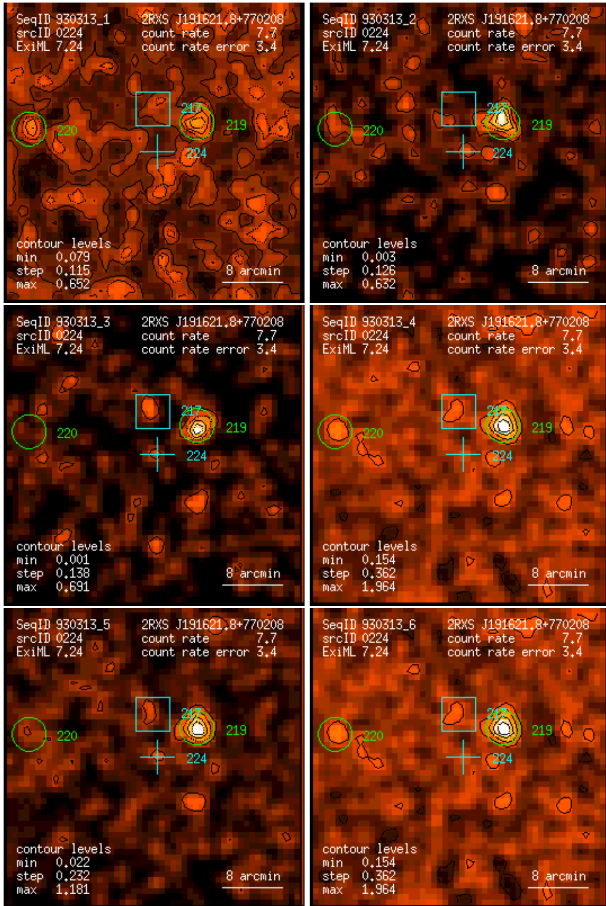
Figure 224: RASS 930313: detection 0224: band rate images, Gaussian filter: (1) PSPC channels 11 – 41, (2) 52 – 90, (3) 91 – 201, (4) 11 – 235, (5) 52 – 201, (6) 11 – 201. Broad band rates in counts/ks. Band rate contour levels in counts/ks/arcmin 2 .
