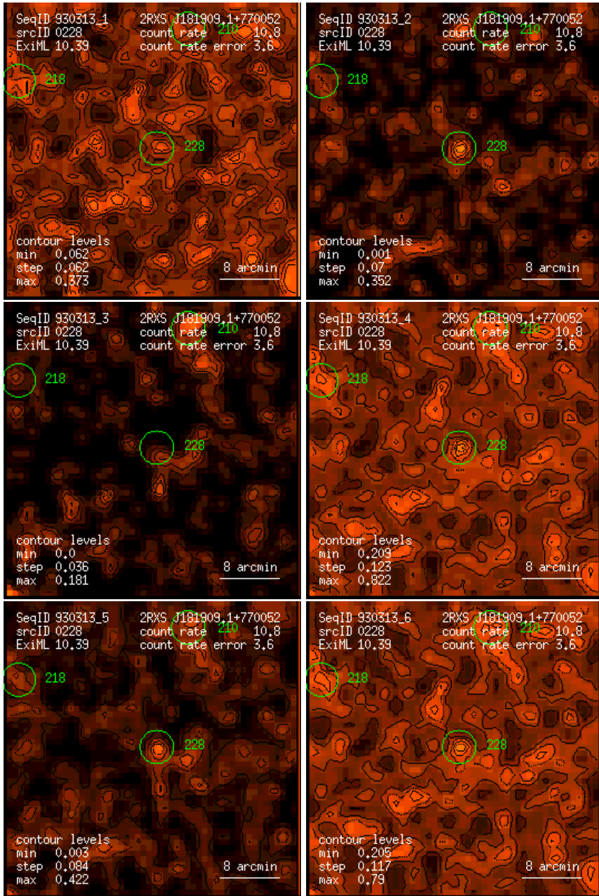
Figure 228: RASS 930313: detection 0228: band rate images, Gaussian filter: (1) PSPC channels 11 – 41, (2) 52 – 90, (3) 91 – 201, (4) 11 – 235, (5) 52 – 201, (6) 11 – 201. Broad band rates in counts/ks. Band rate contour levels in counts/ks/arcmin 2 .
