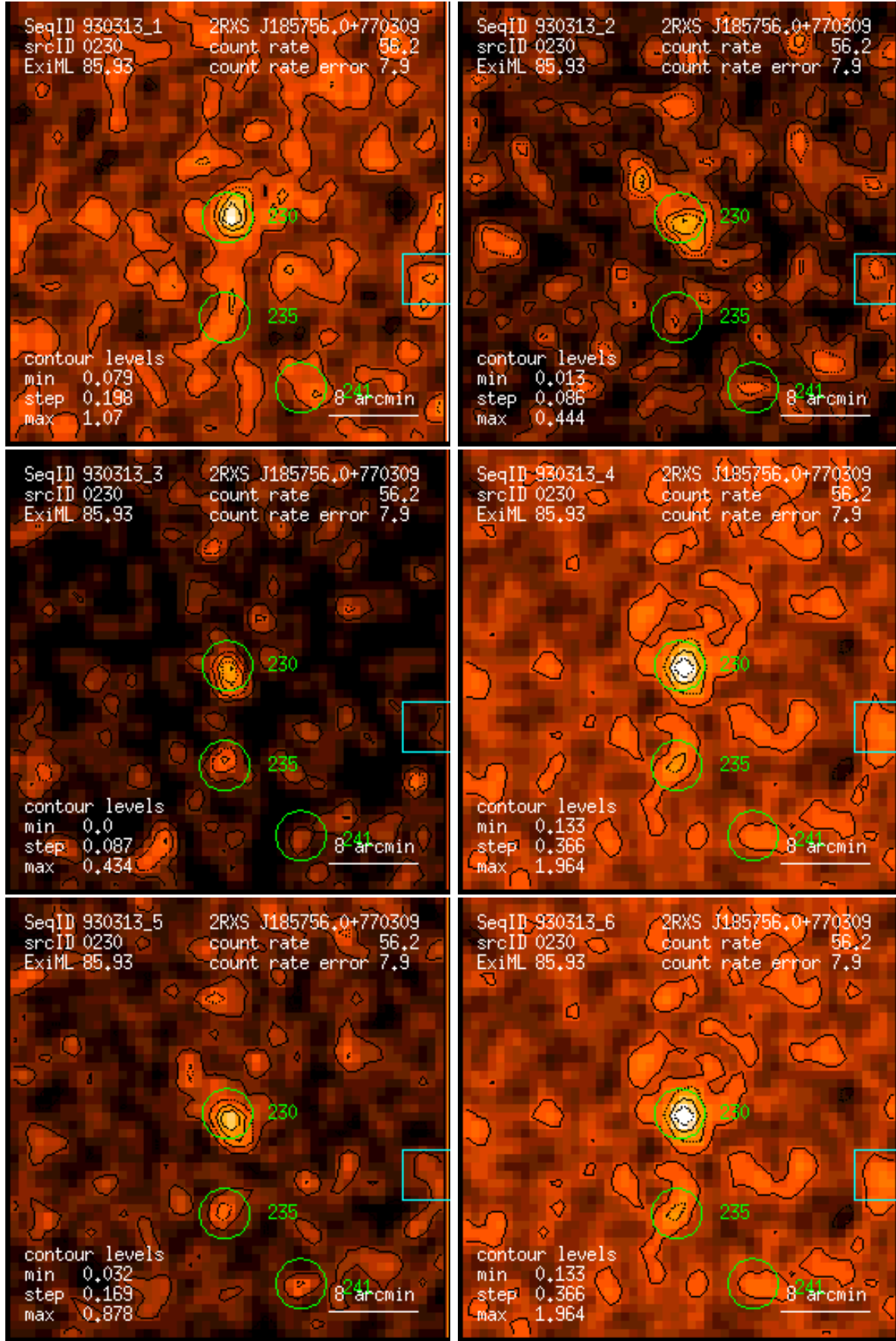
Figure 230: RASS 930313: detection 0230: band rate images, Gaussian filter: (1) PSPC channels 11 – 41, (2) 52 – 90, (3) 91 – 201, (4) 11 – 235, (5) 52 – 201, (6) 11 – 201. Broad band rates in counts/ks. Band rate contour levels in counts/ks/arcmin 2 .
