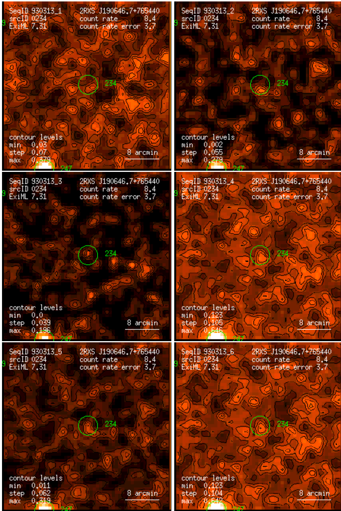
Figure 234: RASS 930313: detection 0234: band rate images, Gaussian filter: (1) PSPC channels 11 – 41, (2) 52 – 90, (3) 91 – 201, (4) 11 – 235, (5) 52 – 201, (6) 11 – 201. Broad band rates in counts/ks. Band rate contour levels in counts/ks/arcmin 2 .
