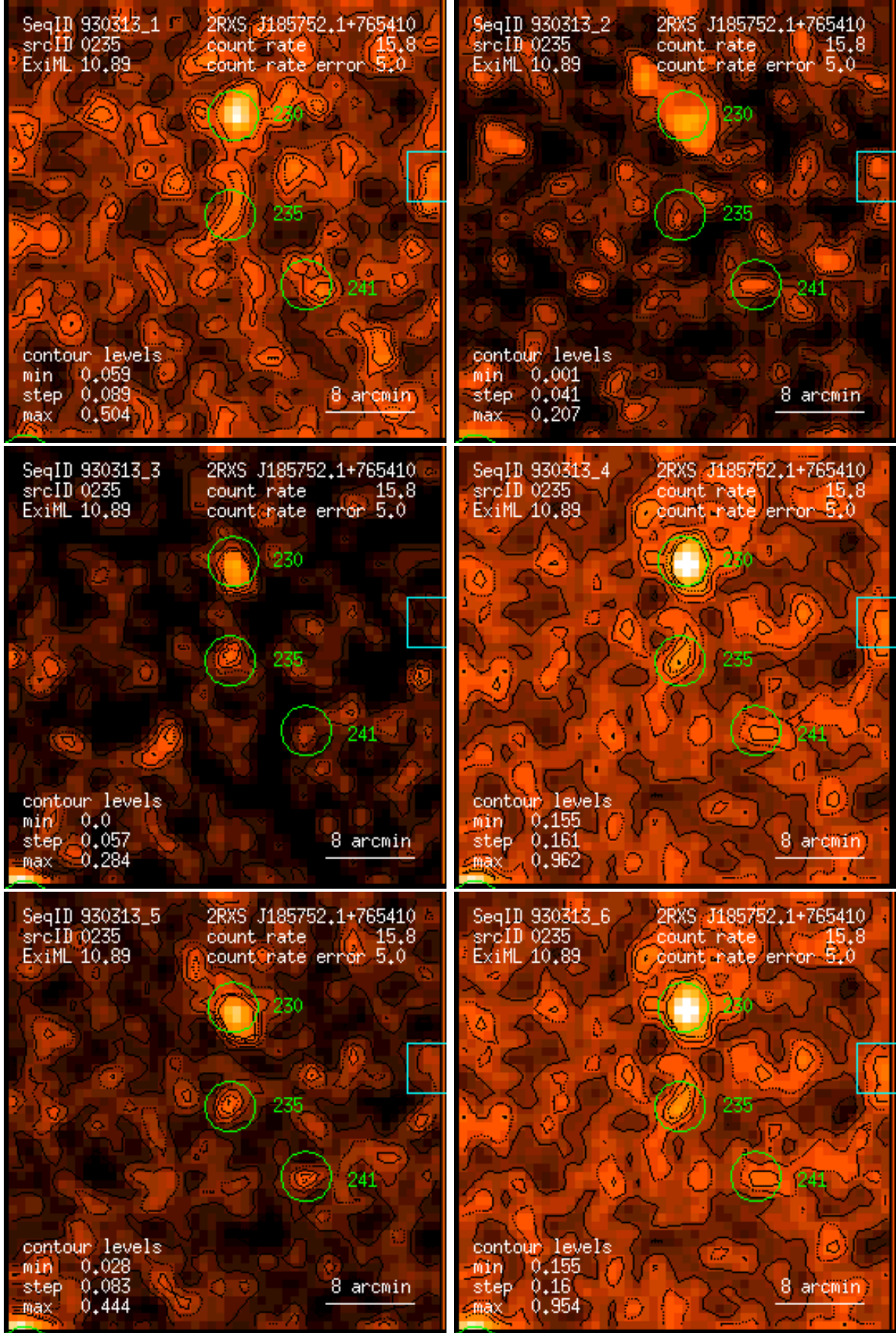
Figure 235: RASS 930313: detection 0235: band rate images, Gaussian filter: (1) PSPC channels 11 – 41, (2) 52 – 90, (3) 91 – 201, (4) 11 – 235, (5) 52 – 201, (6) 11 – 201. Broad band rates in counts/ks. Band rate contour levels in counts/ks/arcmin 2 .
