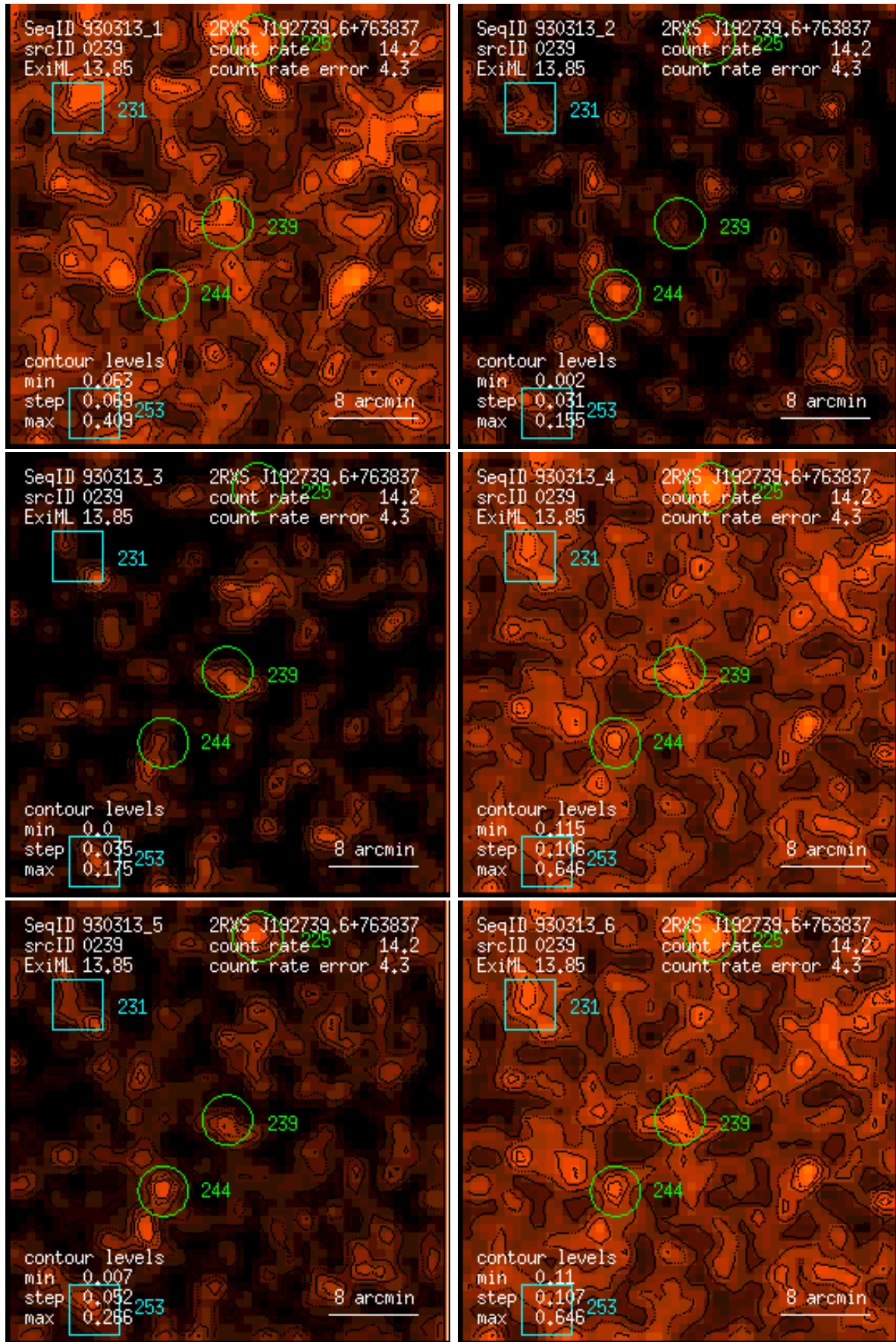
Figure 239: RASS 930313: detection 0239: band rate images, Gaussian filter: (1) PSPC channels 11 – 41, (2) 52 – 90, (3) 91 – 201, (4) 11 – 235, (5) 52 – 201, (6) 11 – 201. Broad band rates in counts/ks. Band rate contour levels in counts/ks/arcmin 2 .
