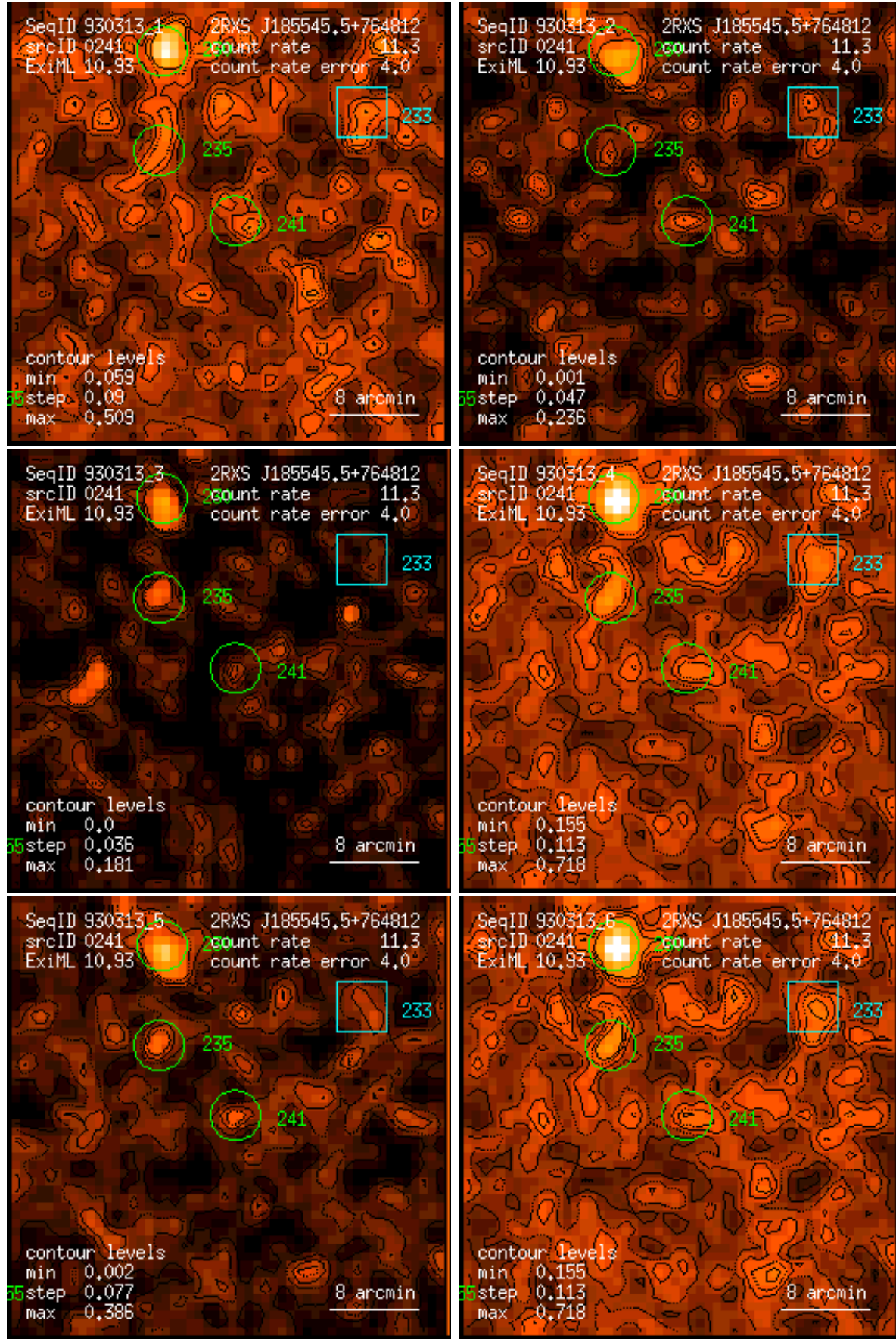
Figure 241: RASS 930313: detection 0241: band rate images, Gaussian filter: (1) PSPC channels 11 – 41, (2) 52 – 90, (3) 91 – 201, (4) 11 – 235, (5) 52 – 201, (6) 11 – 201. Broad band rates in counts/ks. Band rate contour levels in counts/ks/arcmin 2 .
