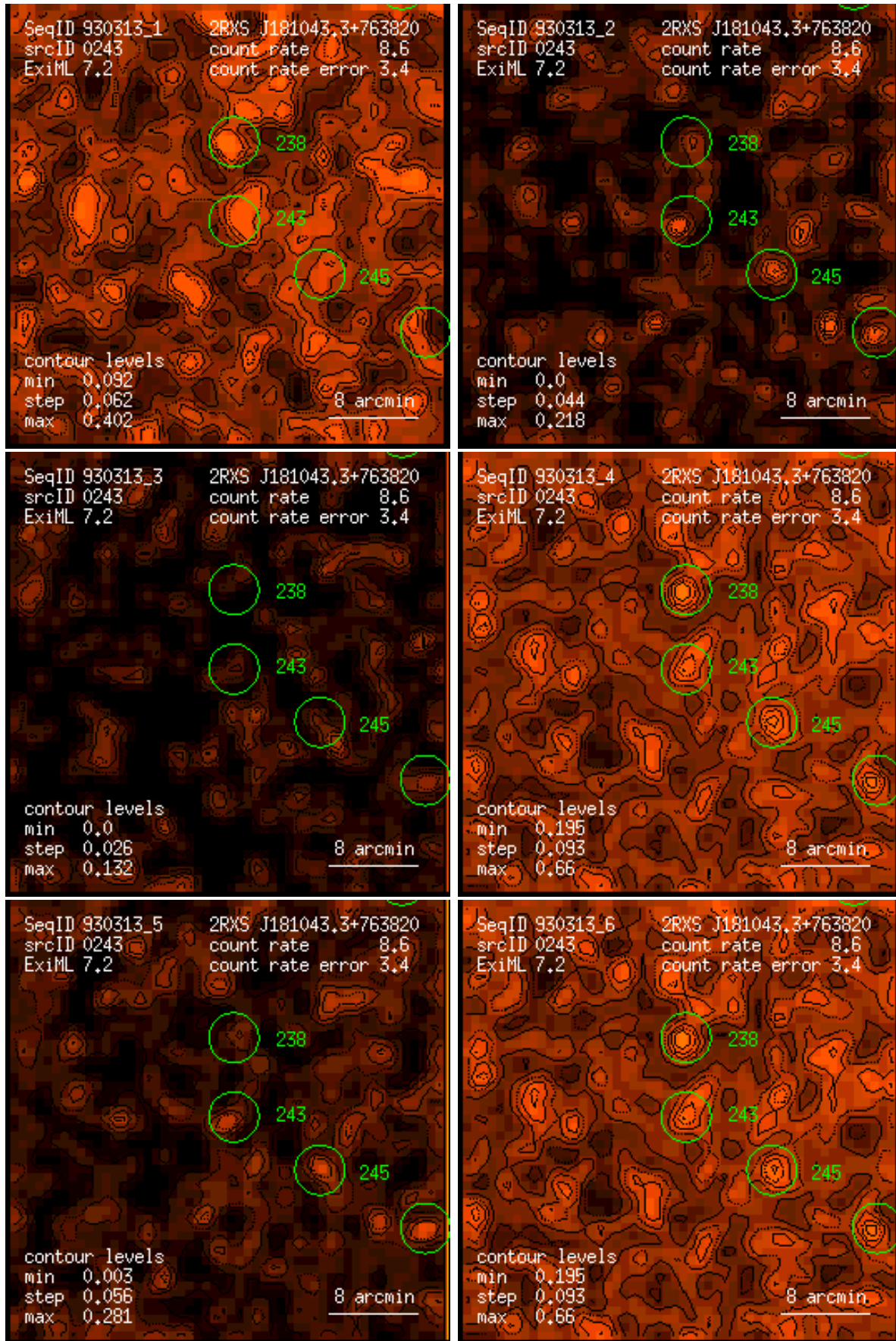
Figure 243: RASS 930313: detection 0243: band rate images, Gaussian filter: (1) PSPC channels 11 – 41, (2) 52 – 90, (3) 91 – 201, (4) 11 – 235, (5) 52 – 201, (6) 11 – 201. Broad band rates in counts/ks. Band rate contour levels in counts/ks/arcmin 2 .
